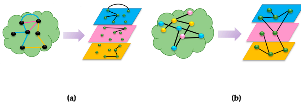
Figure 1. Two categories of multilayered graphs. (a) Edge-colored Graphs (ECG) (b) Node-colored Graphs (NCG).
