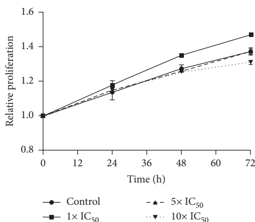
FIGURE 4: Recovery experiment of T. cruzi epimastigotes treated with V^{IV}O(5Brsal)(aminophen) . The growth of parasites exposed for 4 h to 0, 1x , 5x , and 10x IC_{50} V^{IV}O(5Brsal)(aminophen) after compound removal was followed by optic density measures (595 nm) at the indicated time points. Proliferation was determined relative to time zero. Each experiment was performed in triplicate, and the mean and standard deviation were represented for each point.
