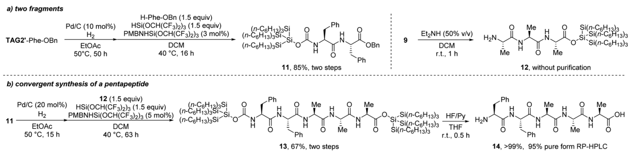
Scheme 10 Convergent synthesis of a pentapeptide (a) preparation of two fragments; (b) convergent connection and removal of the tags.
