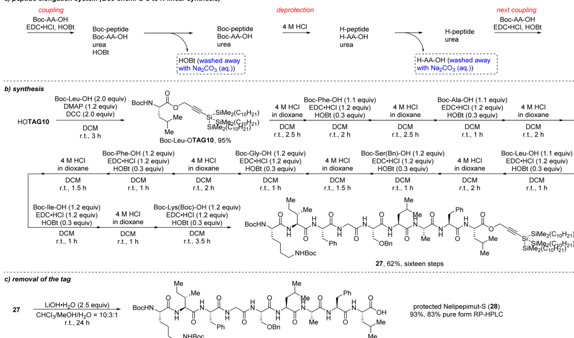
Scheme 14 Synthesis of protected nelipepimut-S with Boc-chemistry (a) peptide elongation system; (b) synthesis with TAG10; (c) removal of the tag.
