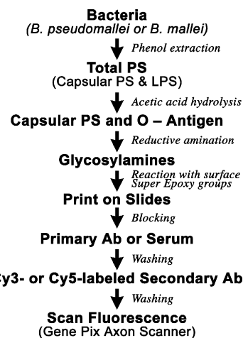
Fig. 1. Flow chart of the generation of Burkholderia polysaccharide microarray.
