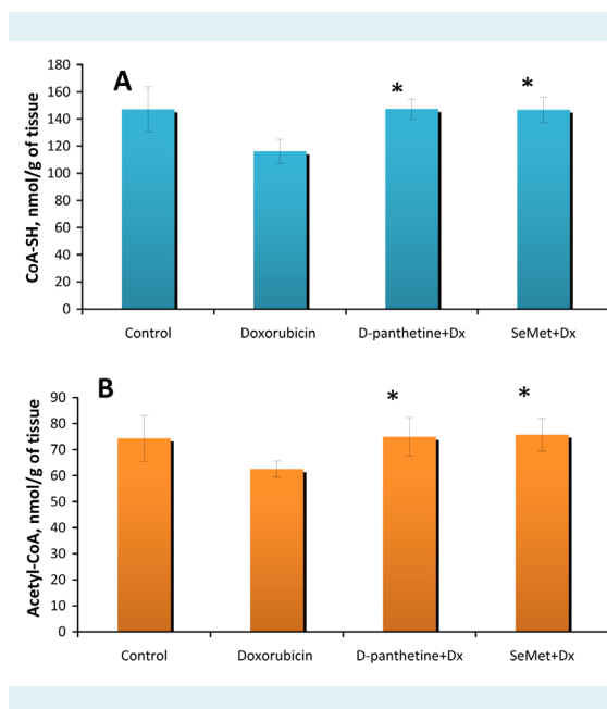
FIGURE 7. Selenomethionine and D-pantethine restore content of coenzyme A-SH ( A ) and acetyl-coenzyme A ( B ) in the liver of normal rats after administration of doxorubicin. * P < 0.05 relative to doxorubicin.
