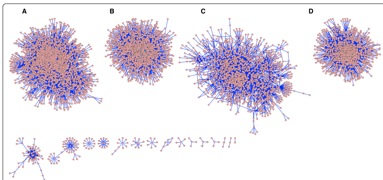
Figure 2 An overview of modules detected in DHN. 19 modules were detected in DHN out of which 4 modules represent ca. 97% of the network. (A) The largest module is enriched for regulation of transcription. (B) The second module with 1540 interconnected proteins representing hormone and hormone receptor signaling pathways. (C) The third module with 1420 proteins enriched for GPCR signaling. (D) The fourth module containing 1312 nodes is enriched for protein translation and induction of apoptosis.
