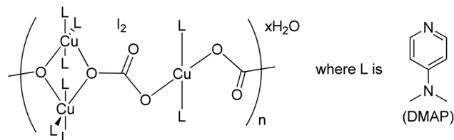
Fig. 2 Structure of the \mu_3 -CO 3 bridged linear polymeric Cu-complex ((Cu 3 (DMAP) 8 (CO 3 ) 2 ) 12 ) n · xH 2 O.
