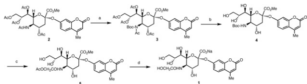
Fig. 1. Synthesis of 4MU-Neu5Gc. (a) Boc 2 O, DMAP, THF, 60 °C, 3 h, 74%; (b) NaOMe, MeOH, 0 °C, 2 h, 78%; (c) (1) TFA, CH 2 Cl 2 , rt, 1 h, (2) AcOCH 2 COCl, NEt 3 , MeOH, 0 °C, 1 h, then rt, 12 h, 69% in two steps; and (d) 0.1 M NaOH, MeOH, 0 °C, 1 h, then rt, 12 h, 49%.
