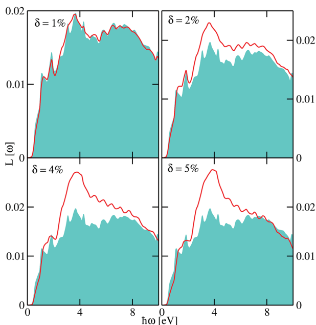
Fig. 5 The low-energy loss spectra of monolayer PbTe at various Te vacancy concentrations \delta as a function of the excitation energy \hbar\omega . The spectra included the effects of electron–hole interactions through the Bethe–Salpeter equation. For reference, we also include the spectra of pristine monolayer PbTe depicted with a turquoise background.
