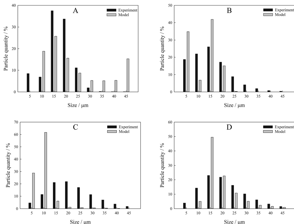
Fig. 6 Particle size distribution bar charts of the studied samples obtained via iterative procedure and experimentally measured. (A) Original Fe 2 O 3 powder; (B) Fe 2 O 3 annealed at 600 °C; (C) Fe 2 O 3 annealed at 700 °C; (D) Fe 2 O 3 annealed at 800 °C.
