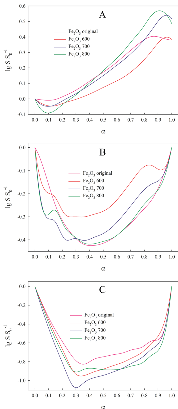
Fig. 5 Optimized relative specific surface area vs. conversion degree curves of oxide forms obtained for 12\text{ }^\circ\text{C min}^{-1} heating rate. (A) \text{Fe}_2\text{O}_3 ; (B) \text{Fe}_3\text{O}_4 ; (C) FeO.
