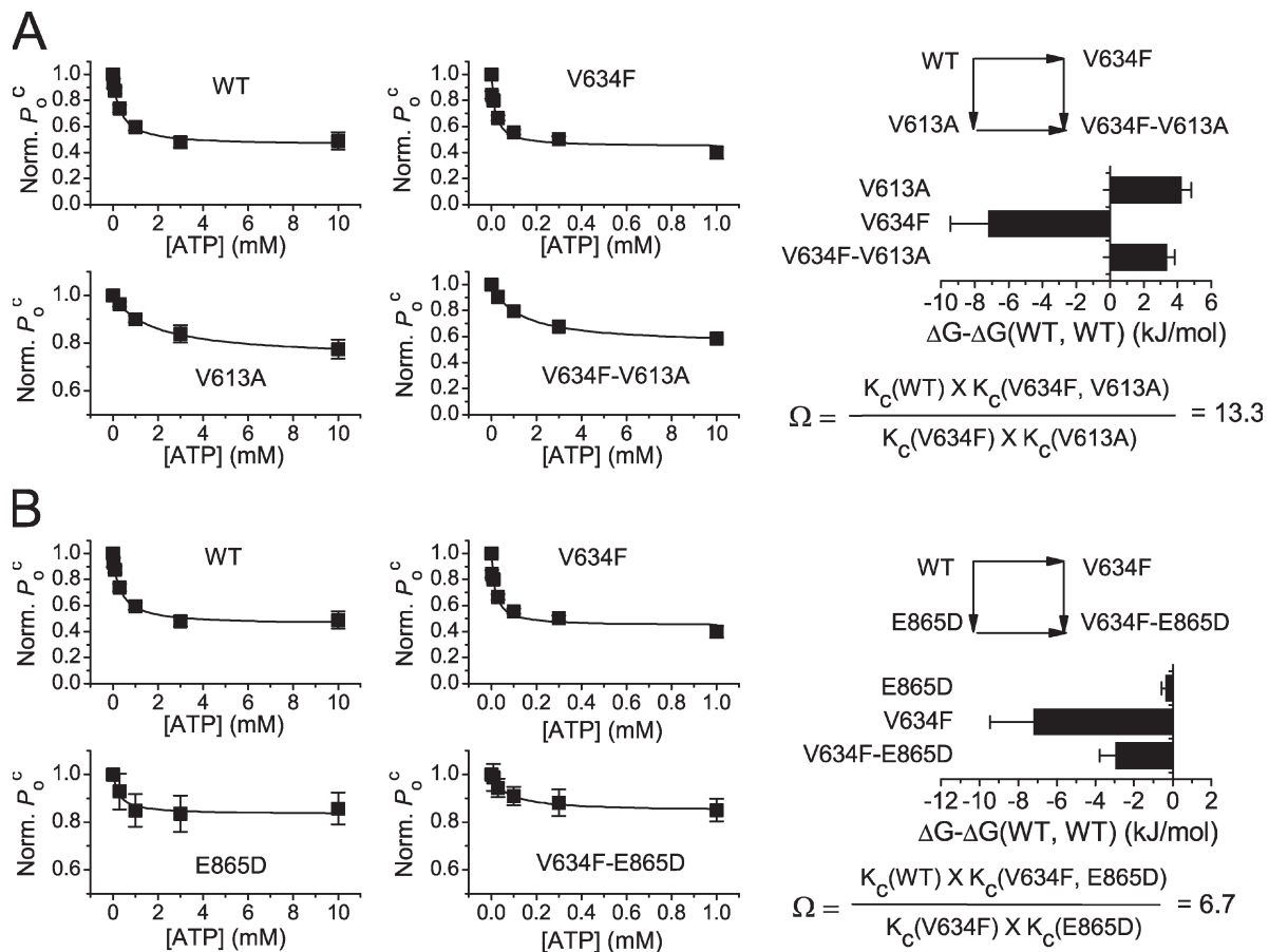
Figure 7. Nonadditive effects of mutations on the ATP modulations of CLC-1. The parameter P_o^c(\text{ATP})/P_o^c(\text{control}) was used as the response to ATP modulation. (A) Mutant cycle analysis of the effects of V634F and V613A mutations on the ATP modulation. ATP dose-response curves of single point mutants and the double mutants were constructed to determine the values of K_o and K_c . The fitted K_c values were used to calculate the free energy differences of single or double mutants (bar graph) according to Eq. 3 and the coupling constant, \Omega , according to Eq. 4. In the context of Eq. 2, the V634F mutation corresponds to the change from X_1 to X_2 , whereas the V613A mutation represents the change from Y_1 to Y_2 . (B) Double mutant cycle analysis for V634F/E865D mutations. The values of \Omega at different voltages are shown in Fig. S2. Error bars represent SEM. n = 4-8 .
