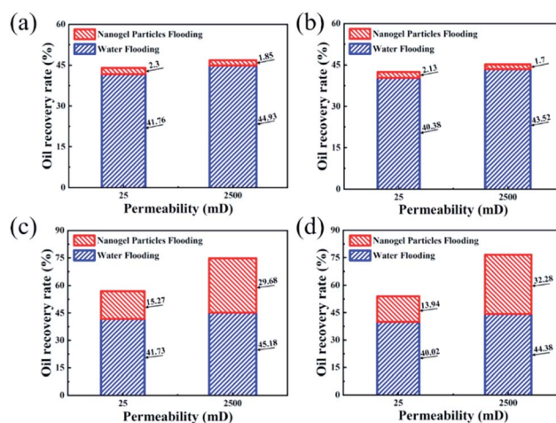
Fig. 6 Oil recovery rates of core flooding experiments versus experimental conditions. (a) 25 mPa s oil and 0.5 wt% nanogel particles; (b) 100 mPa s oil and 0.5 wt% nanogel particles; (c) 25 mPa s oil and 1.5 wt% nanogel particles; (d) 100 mPa s oil and 1.5 wt% nanogel particles.
