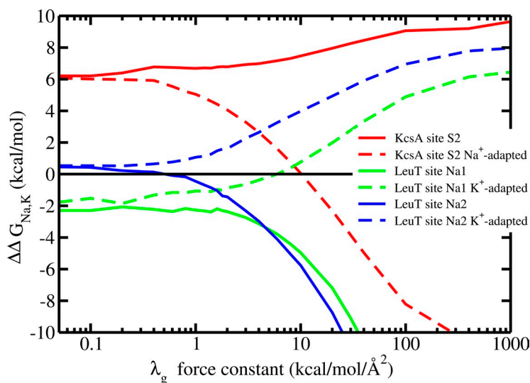
Figure 3. Selectivity in reduced models in which the optimal geometry is adapted to best-fit K^+ or Na^+ (a binding site is K^+ selective when \Delta\Delta G_{Na,K} is positive and Na^+ selective when it is negative). The curves with solid lines correspond to realistic models of KcsA and LeuT, and the curves with dashed lines correspond to putative KcsA and LeuT sites stabilizing an optimal geometry adapted by energy minimization to best-fit Na^+ or K^+ , respectively. Except for the site Na2 of LeuT, the onset of selectivity is established only for very large values of the architectural rigidity \lambda_g , indicating that a fairly stiff geometry is required to counterbalance the inherent trend that is already observed in the confined microdroplet limit ( \lambda_g = 0 ) with loosely restricted ligands. This is adapted from Yu et al. (2010b).
