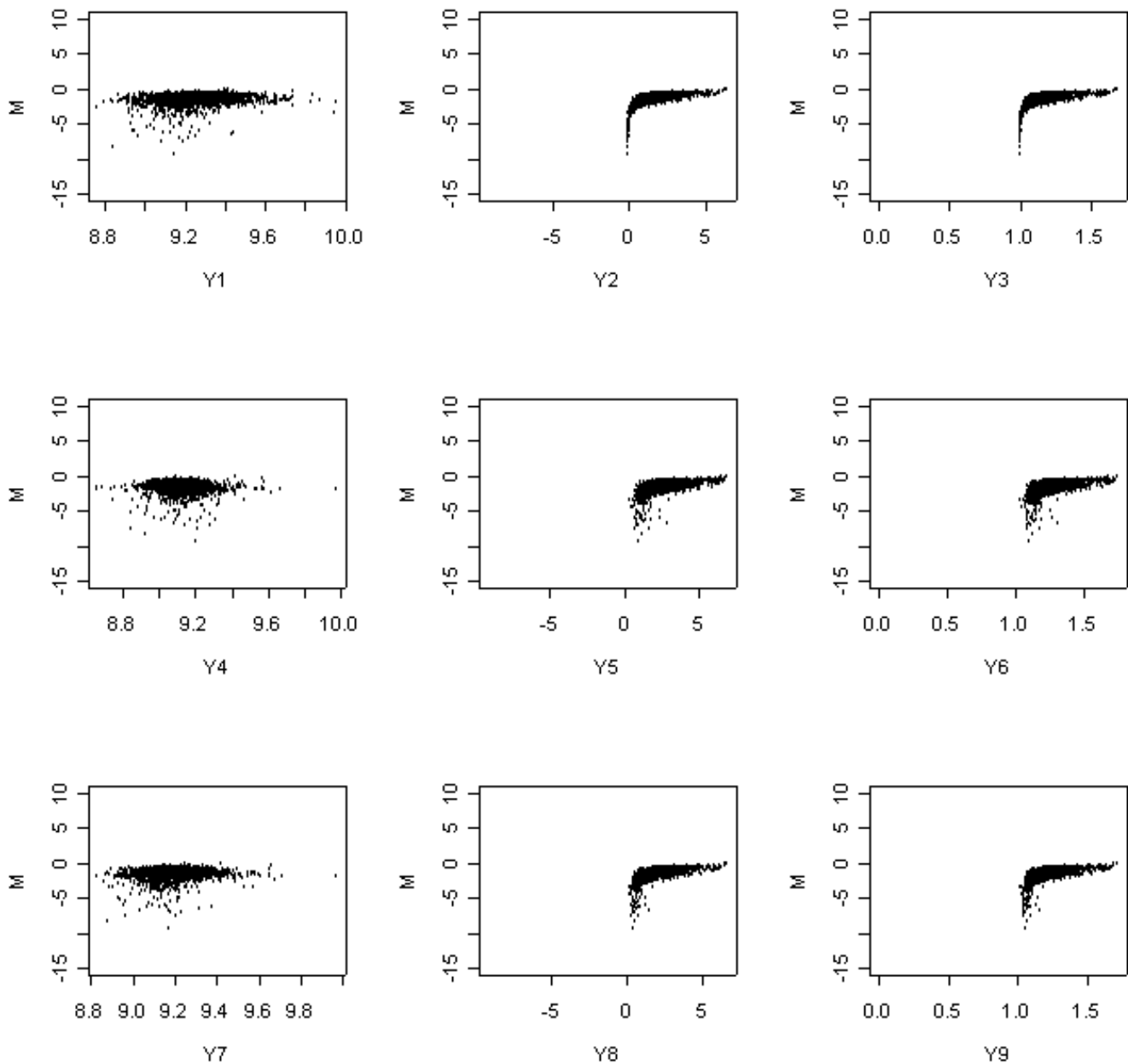
Figure 2 M versus Y_k plots for NCI 60 data; the correlation coefficient of M = \log(R/G) and Y_k 's ( k = 1, \dots, 9 ) are 0.2025, 0.6238, 0.6256, -0.0184, 0.5065, 0.5096, 0.1291, 0.5707, and 0.5729, respectively.
