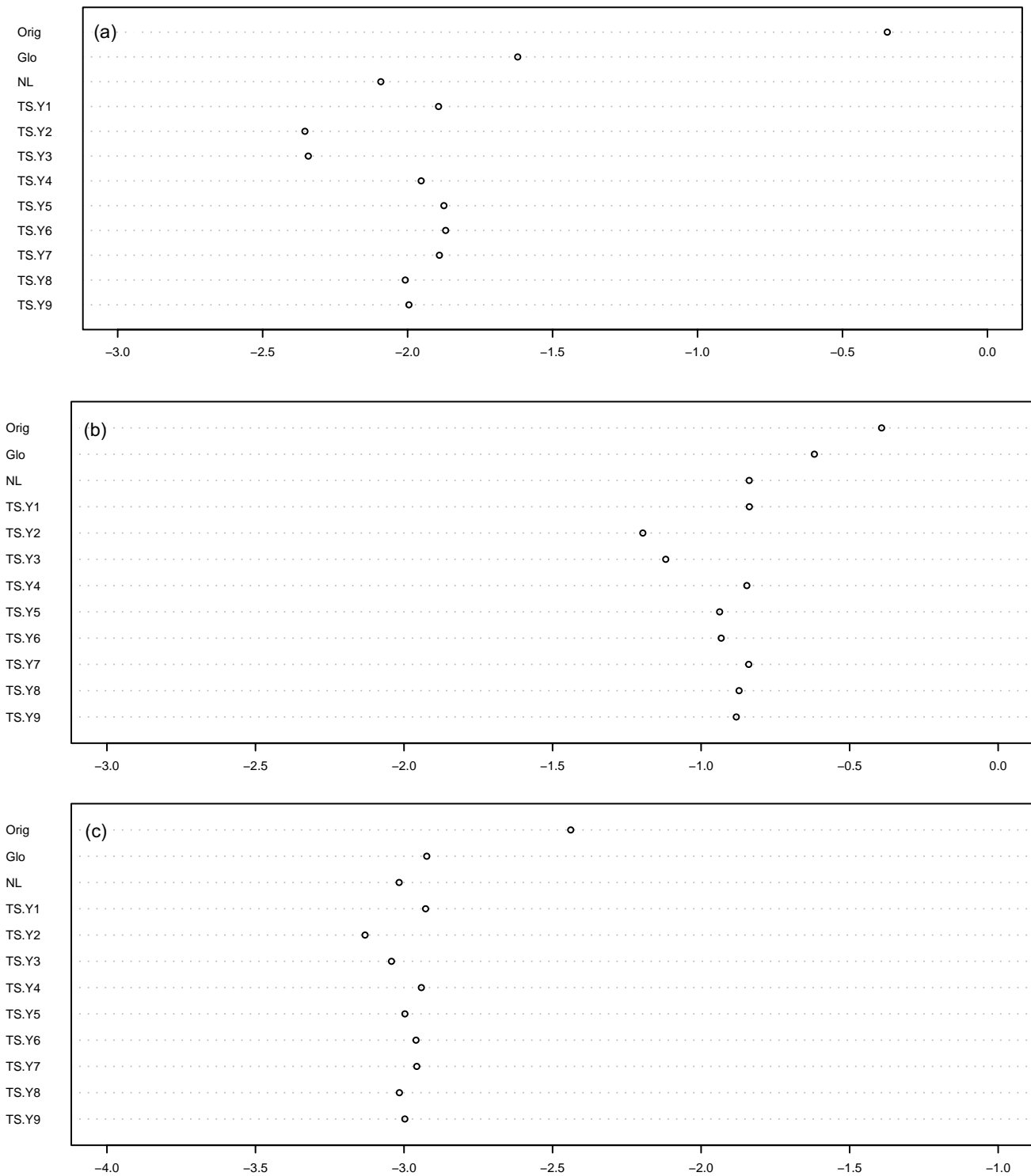
Figure 5 Dot plots of log-transformed variance estimates. Y-axis represents normalization methods and the X-axis represents the mean value of log-transformed variance estimates. (a) Colorectal cancer data set from NCI 60 (b) Cortical Stem Cells Data (Park et al. [17]) (c) Kidney data (Pritchard et al. [18]).
