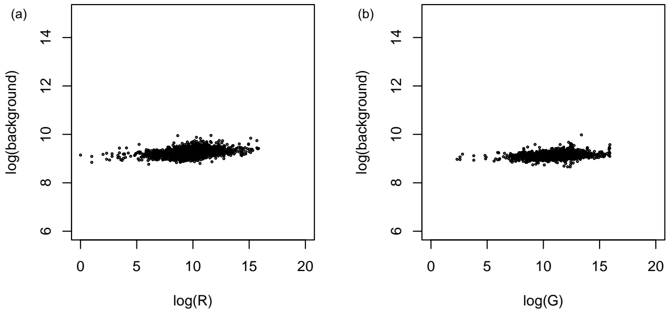
Figure 1 Example of correlations between background intensity and signal intensity from one of the NCI 60 data of Zhuo et al. 16 (a) \log(\text{background}) vs. \log(R) , correlation coefficient: 0.353, (b) \log(\text{background}) vs. \log(G) , correlation coefficient: 0.232.
