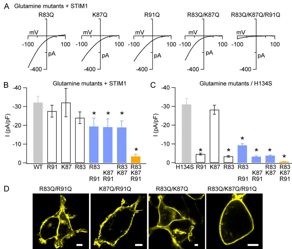
Figure 5. The polarity of the basic domain also contributes to Orai1 channel opening. (A) I–V relationships of Gln Orai1 mutants in 20 mM Ca 2+ Ringer’s solution. (B and C) Summary of the peak current amplitudes (I [pA/pF]) of WT and Gln Orai1 mutants activated by STIM1 (B), or by the GOF H134S mutant (C). Unlike the equivalent Ser mutants (Fig. 2 C), the Gln mutants are more strongly activated by STIM1, suggesting that increased polarity of Gln relative to Ser promotes Orai1 channel opening. Note that K87Q/H134S mutation had no detrimental effect on Orai1 current density. Values are mean ± SEM (n = 6–9 cells per condition; *, P < 0.05, Student’s t test). (D) Expression of the indicated Q mutants in the plasma membrane. Scale bars, 5 μm.
