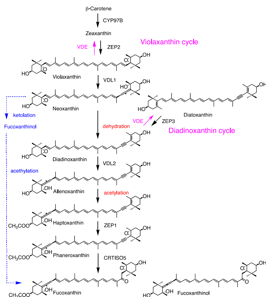
Figure 5. Carotenogenesis pathway from \beta -carotene to fucoxanthin, as well as violaxanthin and diadinoxanthin cycles in the brown alga Phaeodactylum tricornutum . VDE is activated by high-light conditions. The dotted blue line highlights a simple pathway (Figure 1). The illustrated structures of fucoxanthin and fucoxanthinol are reversed for the right and left sides according to the IUPAC-IUB semi-systematic rule.
