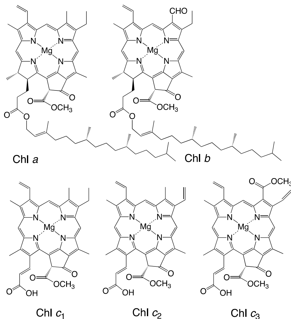
Figure 1. Structures of chlorophylls (Chls).
