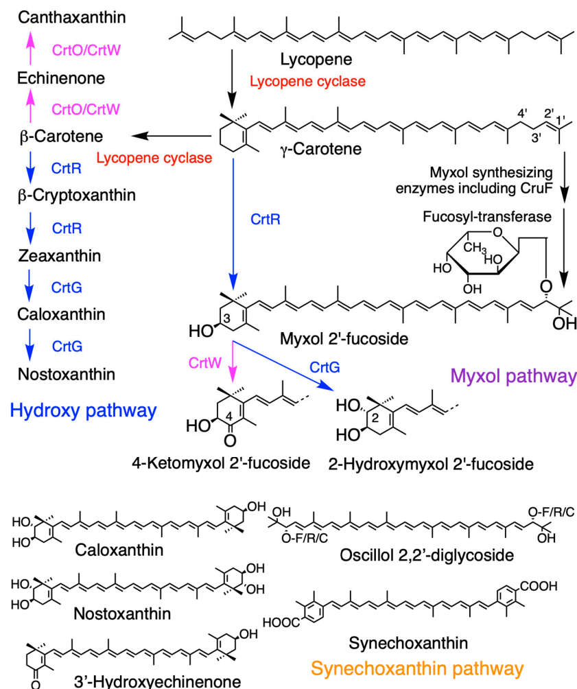
Figure 3. Major carotenogenesis pathways in cyanobacteria along with the functionally confirmed enzymes involved. These pathways and enzymes vary across cyanobacterial species. Two lycopene cyclases, CruA and CrtL, have been identified. The glycoside attached to myxol and oscillol may be fucose, rhamnose, or chinovose. This figure is an updated version presented in the previous review [3].
