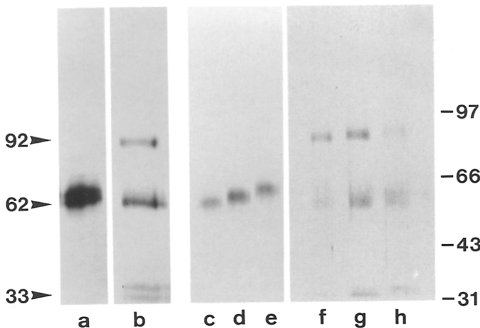
Figure 4. Analysis of the 64-kD scatter factor by electrophoresis on reducing SDS polyacrylamide gels. Purified scatter factor was analyzed on nonreducing (a) and reducing SDS polyacrylamide gels (b). The nonreduced 64-kD band splits into components with apparent molecular masses of 92-, 62-, and a doublet of 34/32-kD. The broad nonreduced 64-kD band (a) was cut into three pieces with increasing molecular mass and the electroeluted material was analyzed by electrophoresis on nonreducing (c–e) and reducing (f–h) SDS gels (5–15% linear gradients). It can be seen that the material with the lowest molecular mass (c) contains mostly the 92-kD component (f), whereas the fraction with the highest molecular mass (e) is mainly composed of the 62- and 34-kD components (h). Molecular mass markers are as in Fig. 2. Analysis of scatter factor activity revealed that the three eluates (c–e) exhibited the same specific activity, i.e., scanning of the protein bands resulted in ratios of 1:1.9:1.4, whereas the ratios of activity were 1:2.0:1.5.
