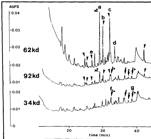
Figure 6. HPLC analysis of tryptic peptides of the 92-, 62-, and 34-kD components of scatter factor. The proteins, blotted onto PVDF membranes, were digested with trypsin in situ, and the released peptides analyzed by reversed phase HPLC (see Materials and Methods). Absorbance of peptides at 214 nm was recorded (AUFS; absorbance units, fraction of full scale). Arrowheads and arrows mark peptide pairs with identical elution properties of the 92- and 62-, and the 92- and 34-kD components, respectively. Asterisks mark the peptide pairs of the 92- and 62-, and of the 92- and 34-kD proteins, respectively, which exhibit an identical amino acid sequence. The sequences of peptides a-g were used for the homology search.
