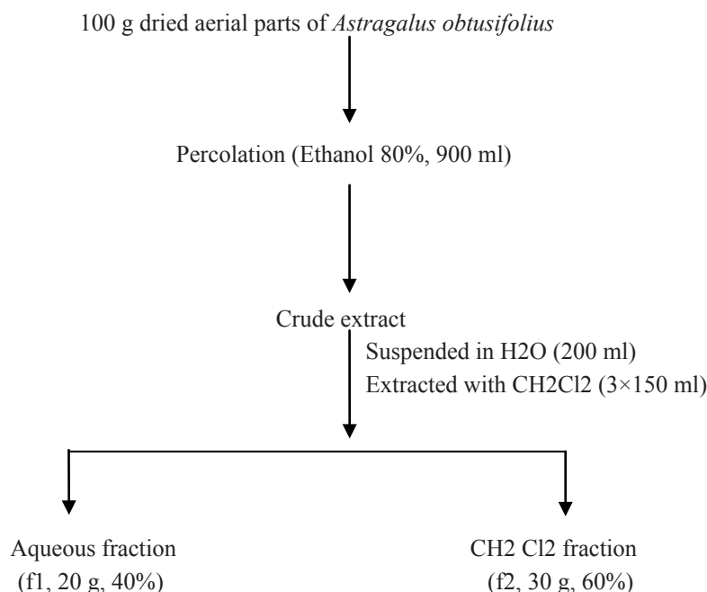
Figure 1. Flow diagram of fractionation of the crude extract obtained from the aerial parts of Astragalus obtusifolius .
