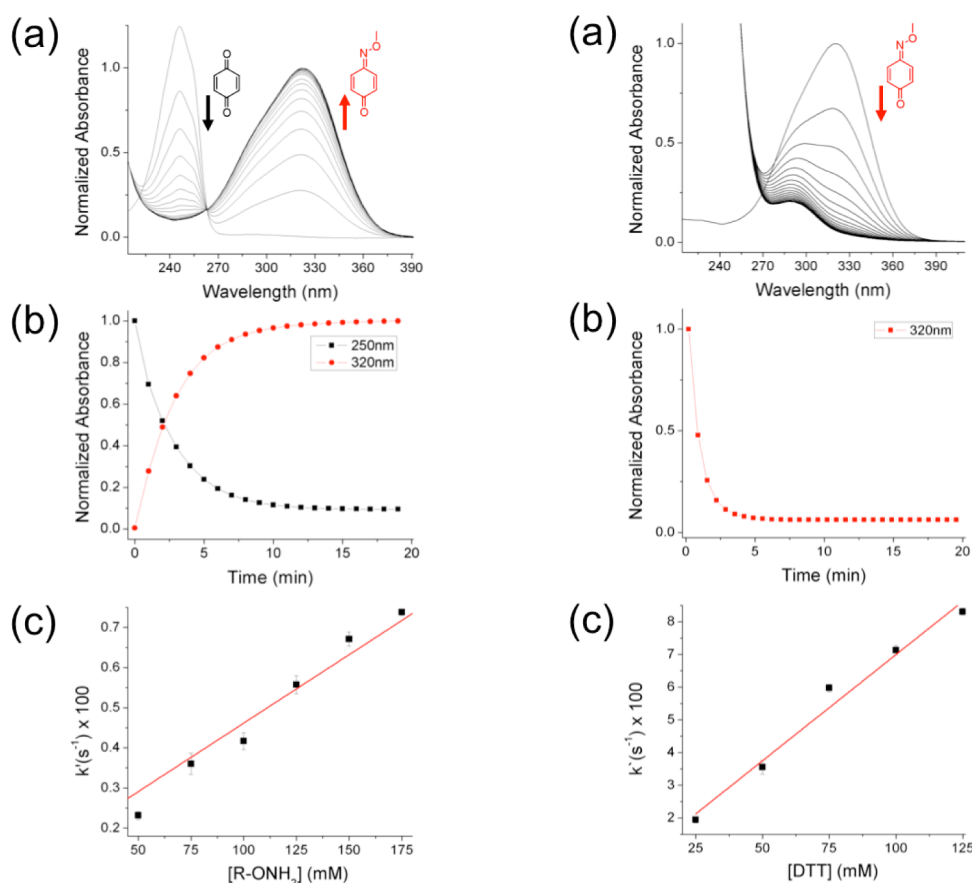
Figure 2. Kinetics of CRRL conjugation between BQ (200 \mu\text{M} ) and methoxyamine (100 mM), and cleavage of QO (200 \mu\text{M} ) with dithiothreitol (DTT) (100 mM), determined by UV-vis spectroscopy. (Left) (a) UV-vis spectra showing the conversion from BQ (248 nm) to QO (320 nm) with a clear isobestic point. (b) A plot of absorbance maxima versus time for BQ and QO. An exponential increase of QO and decay of BQ are fitted to pseudo-first-order kinetics to obtain k' ( 4.2 \times 10^{-3} \text{ s}^{-1} ). (c) A plot of k' versus varying [\text{CH}_3\text{-ONH}_2] to determine the second-order rate constant k for the reaction of BQ with \text{CH}_3\text{ONH}_2 to generate QO. The rate constant for CRRL conjugation is 3.4 \times 10^{-2} (\pm 6.5 \times 10^{-4}) \text{ M}^{-1} \text{ s}^{-1} . (Right) (a) UV-vis spectra characterization for the cleavage reaction versus time (QO, 320 nm; AP, 292 nm). (b) A plot of QO (200 \mu\text{M} ) absorbance (320 nm) versus time in the presence of the reductant DTT (10 mM) follows a pseudo-first-order exponential decay ( k' = 7.3 \times 10^{-2} \text{ s}^{-1} ). (c) A plot of k' versus varying [DTT] to determine the second-order rate constant k for the cleavage of QO to generate AP. The CRRL cleavage rate constant k = 6.5 \times 10^{-1} (\pm 3.0 \times 10^{-2}) \text{ M}^{-1} \text{ s}^{-1} .
