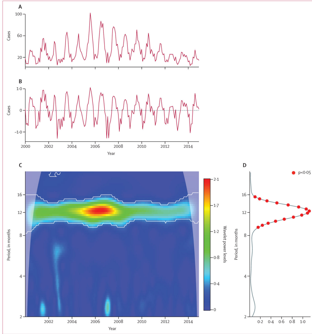
Figure 2. Wavelet analysis for Neisseria meningitidis in South Africa, 2000–14 (A) Raw time-series of reported cases. (B) Log-transformed, detrended, and standardised time-series used for wavelet analysis. (C) Wavelet power spectrum: wavelet power values increase from blue to red, and white contour lines indicate the 5% significance level. In this example, the time-series shows a significant 12 month periodicity over the entire time period. Shaded regions on either end delimit the cone of influence, where edge effects become important and spectral information is less robust. (D) Average wavelet power over time, with red dots indicating significant periods at the 5% level. Here the significant peak of power occurred at the 12 month period. Additional details and analyses for all other countries are available in the appendix.
