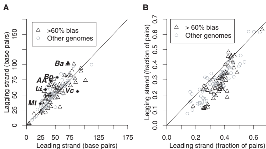
Figure 4. Across 139 chromosomes from 130 bacteria, adjacent pairs of genes on the leading and lagging strands are separated by similar distances, but pairs on the leading strand are more conserved. (A) The median distance between pairs on the leading strand (x-axis) and the lagging strand (y-axis). (B) The proportion of pairs that are conserved within 5 kb in a distant genome, on both strands (same axes). The lines show x = y . In (A), a few chromosomes do have significantly different distributions of distances on the two strands (false discovery rate < 0.05 ) and are indicated with labels and filled diamonds: 'Ba', Bacillus anthracis Ames strain and Ames ancestor strain; 'Bp', Burkholderia pseudomallei K96243 chromosome 2; 'AA', Acinetobacter sp. ADP1; 'Li', Leptospira interrogans serovar Copenhageni strain Fiocruz L1-130 chromosome 1; 'Mt', Mycobacterium tuberculosis H37Rv; and 'Vc', Vibrio cholerae chromosome 2. In (B), none of the chromosomes has significantly greater conservation of pairs on the lagging strand (the points above the line are not significantly different from equality, all P > 0.05 , Fisher's exact test).
