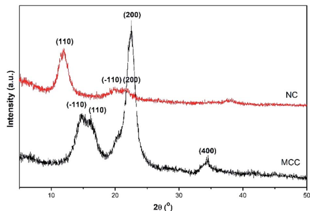
Fig. 3 XRD spectra of MCC and NC.
