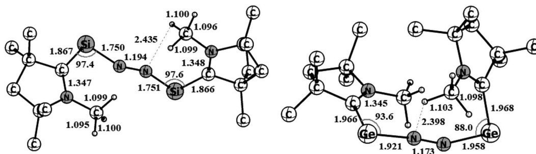
Fig. 3 Optimized equilibrium geometries of (\text{cAAC-Si})_2(\text{N}_2) (1) and (\text{cAAC-Ge})_2(\text{N}_2) (2) in singlet states at the BP86-D3(BJ)/TZ2P level of theory.
