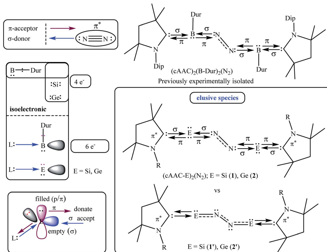
Fig. 2 The isoelectronic analogies of B-Dur, and (L)(B-Dur) with E, and (L)E [E = Si, Ge] (left), previously reported (\text{cAAC})_2(\text{B-Dur})_2(\text{N}_2) (top, right), and elusive species (\text{cAAC-E})_2(\text{N}_2) (1–2; E = Si, Ge) (right, bottom).
