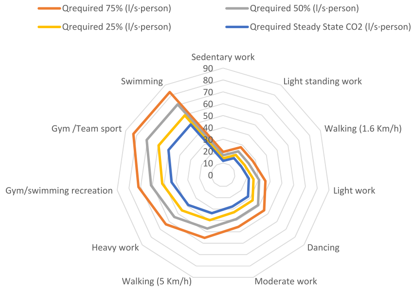
Fig. 1. Required ventilation flow by activity.
