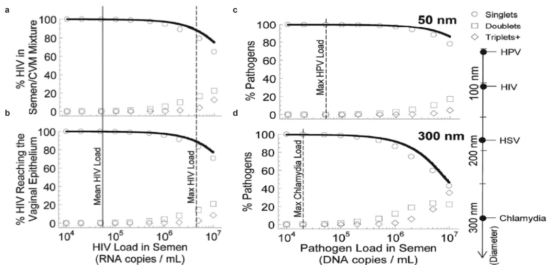
Figure 4. Simulations of virion collisions at different viral loads and particle sizes. The fraction of virions over the first 12 hours post ejaculation as a function of virion density in semen which have undergone no collision (singlets), one collision (doublets) or two or more collisions (triplets+) for all HIV virions (a) in semen/CVM mixture and (b) that have reached the vaginal epithelium. (c–d) The fraction of (c) 50 nm pathogens and (d) 300 nm pathogens in diameter that have diffused across CVM and reached the vaginal epithelium. Solid line represents an exponential function approximation of the virion load arriving at the epithelial layer that experiences no collisions with other virions. Modified and reproduced under creative commons license from. 68
