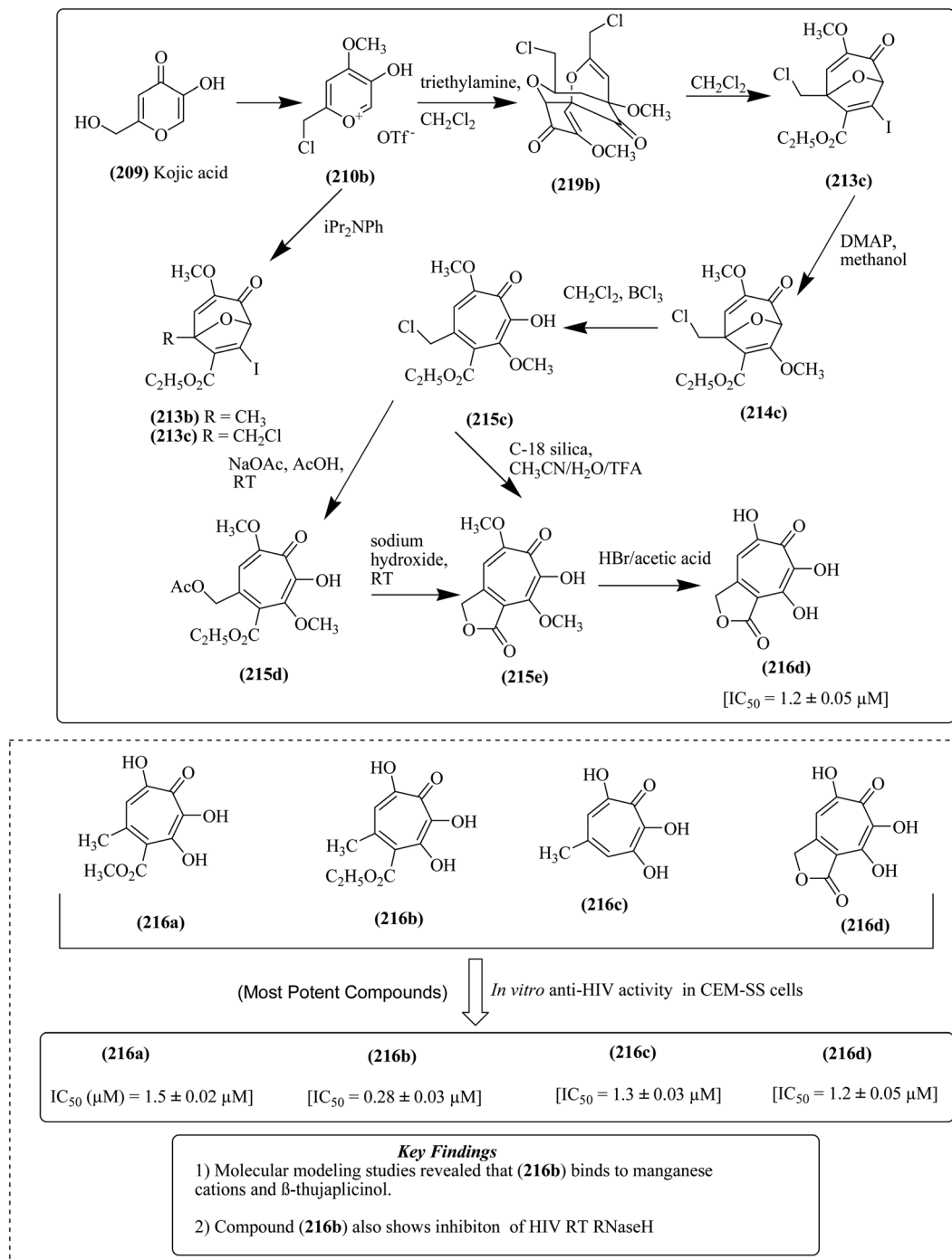
Fig. 28 Synthesis of 3,7-dihydroxytropolone analogs together with important key findings of the potent compounds.
