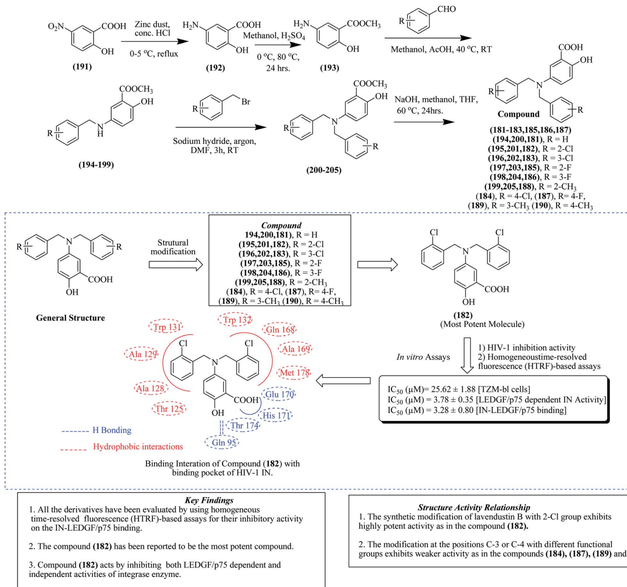
Fig. 21 Structures of lavendustin B analogs together with their docking features.
