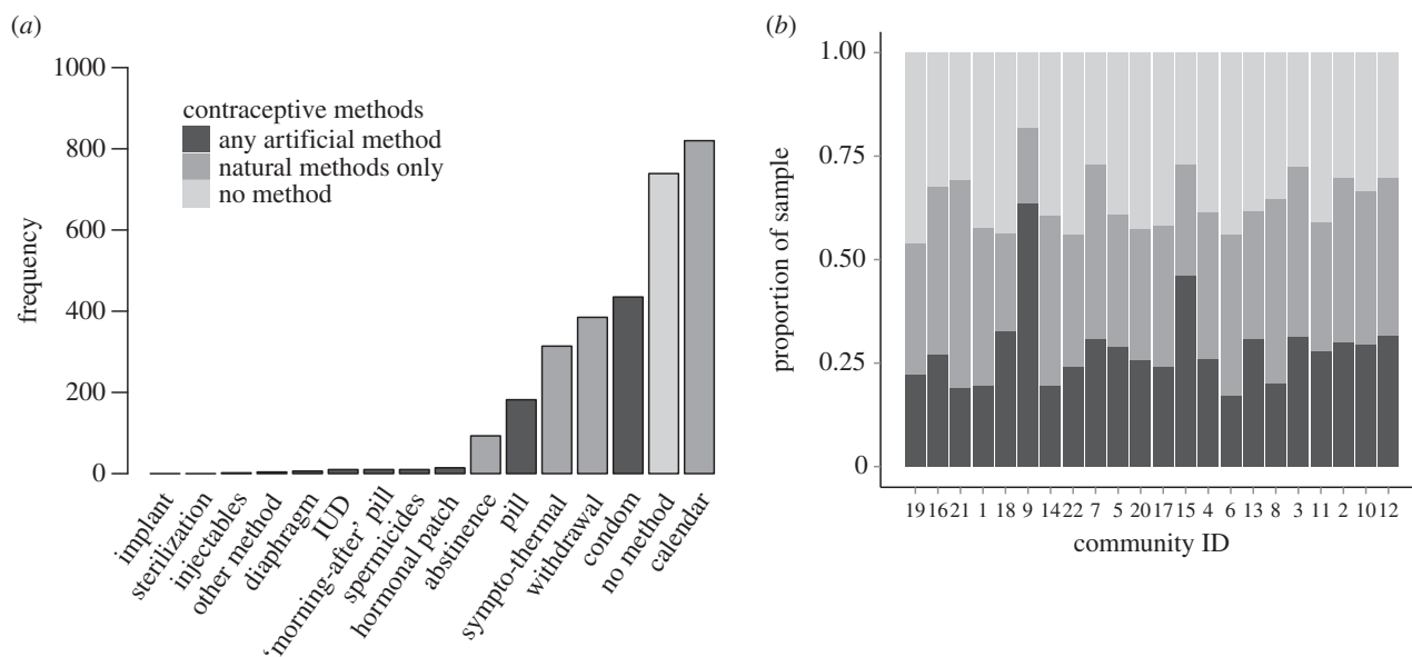
Figure 1. Frequency distributions of (a) contraceptives ever used by women in the sample ( n = 1972 ) and (b) proportion of women using the different method types. Bars in (b) are ordered in terms of increasing population density from left to right. Community IDs give the order in which the communities were sampled.
