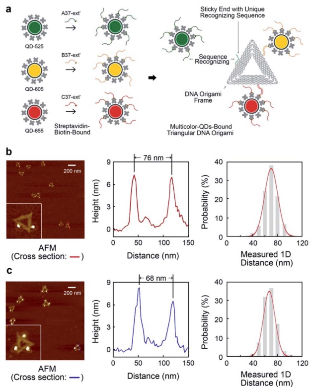
Fig. 2 Multivalent triangular DNA origami with multicolour quantum dots assembly. (a) Schematic showing synthesizing multivalent optical moieties on single DNA origami via unique sequence recognizing the sticky ends on each side of DNA origami and the ssDNA bound to QDs. QD-525, QD-605 and QD-655 were attached in the 3-QDs-bound system. The certain position of chosen quantum dot can be spatially controlled. (b) The characterization of 2-QDs-Bound DNA origami. AFM images with cross-section reveal the distances between quantum dots on a single DNA origami. Distribution of inter-QDs distances shows the statistics of spatially controlled quantum dots on DNA origami. (c) The characterization of 3-QDs-bound DNA origami with AFM scanning, cross-section analysis and QDs spatial distribution.
