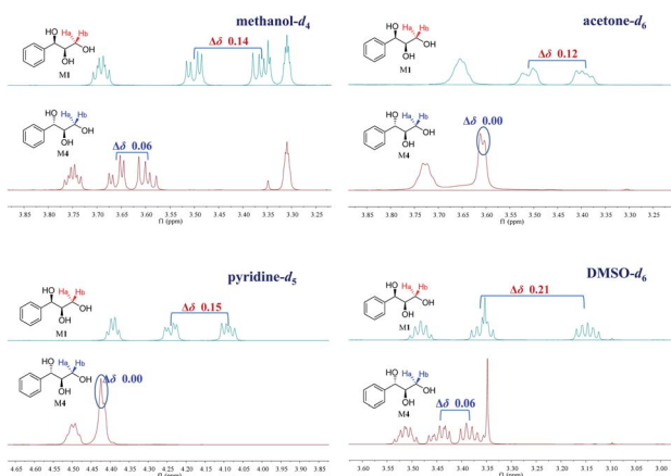
Fig. 3 Influence of different deuterated solvents on the \Delta\delta_{\text{H}3\text{a}-\text{H}3\text{b}} values of M1 and M4 ( ^1\text{H} NMR 500 MHz).
