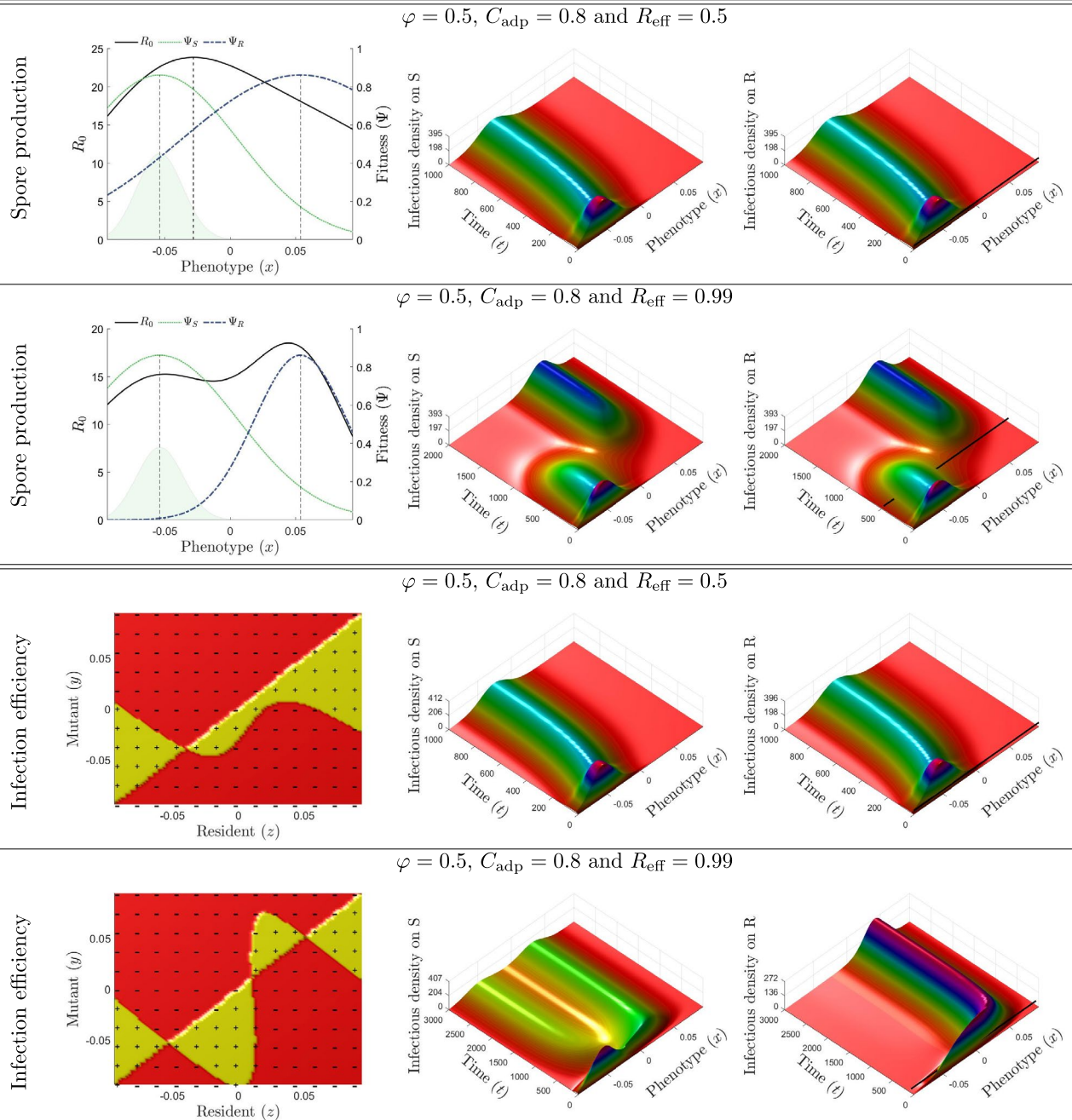
FIGURE 2 Evolutionary epidemiological dynamics. Line 1. The resistance impacts only spore production. The fitness function is unimodal (left panel). At t = 0 , the pathogen population is at its mutation–selection equilibrium on the S cultivar (light green distribution). The infection dynamics and phenotypic composition of the pathogen population on the S and R cultivars are displayed in the central and right panels, respectively. The black line in the right panel corresponds to the time to emergence T_{\text{emg}} . Line 2. As in line 1, but with R_{\text{eff}} = 0.99 . The fitness function is bimodal, with both a global and a local maximum. Line 3. The resistance affects only infection efficiency. The pairwise invasibility plot (PIP) visualizes the sign of invasion fitness f_x(y) (left panel). As a mutant strain y will invade the resident population x only if f_x(y) > 0 , the PIP reveals a single evolutionary attractor \mu^* (the vertical line through \mu^* , is completely contained within a region marked “–”). Line 4. As in line 3 but with R_{\text{eff}} = 0.99 . The PIP reveals two evolutionary attractors (left panel). For all panels, all the other parameters are set to their reference values (Table 2). Note that the timescale axis varies between lines
