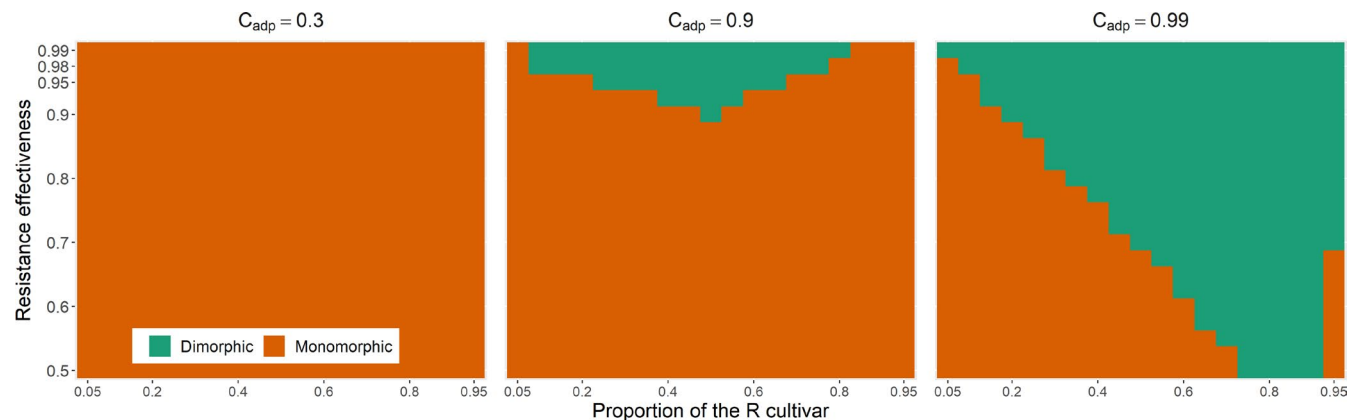
FIGURE 3 Nature of the evolutionary equilibrium (monomorphic or dimorphic) when the resistance affects only infection efficiency. The nature of the equilibrium is characterized as a function of the proportion of the R cultivar at planting (x-axis) and of the relative effectiveness of the resistant cultivar (y-axis) for three costs of adaptation (columns). For all panels, all the other parameters are set to their reference values (Table 2)
