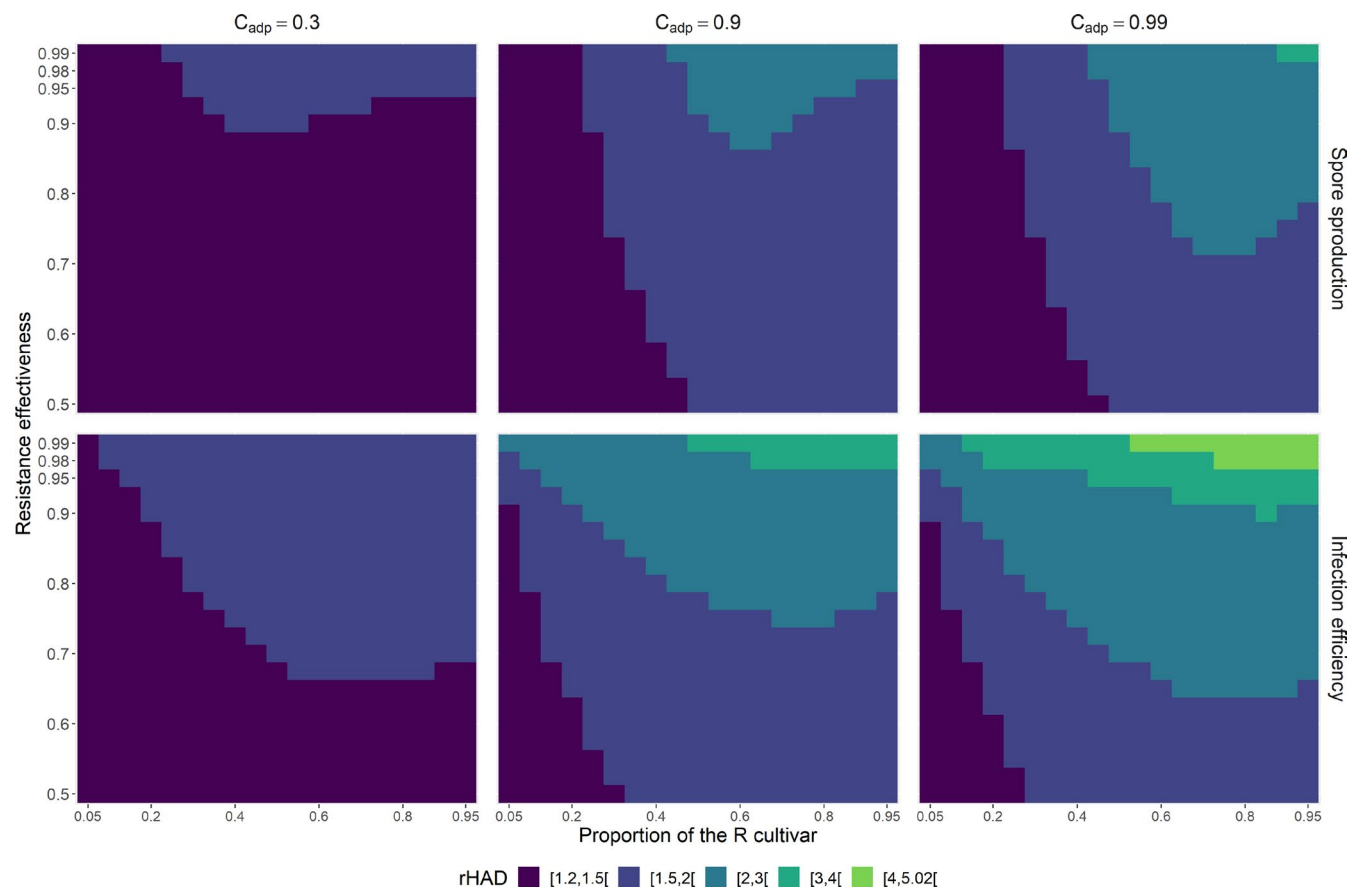
FIGURE 5 Epidemiological outcomes. Epidemiological control is estimated by calculating the gain in relative healthy area duration (rHAD), a proxy for crop yield. Line 1. The resistance affects only total spore production (SP scenario). Epidemiological control is characterized as a function of the proportion of the R cultivar at planting (x-axis) and of the relative effectiveness of the resistant cultivar (y-axis) for three costs of adaptation (columns). Line 2. As in line 1 when the resistance affects only infection efficiency (IE scenario). For all panels, all the other parameters are set to their reference values (Table 2)
