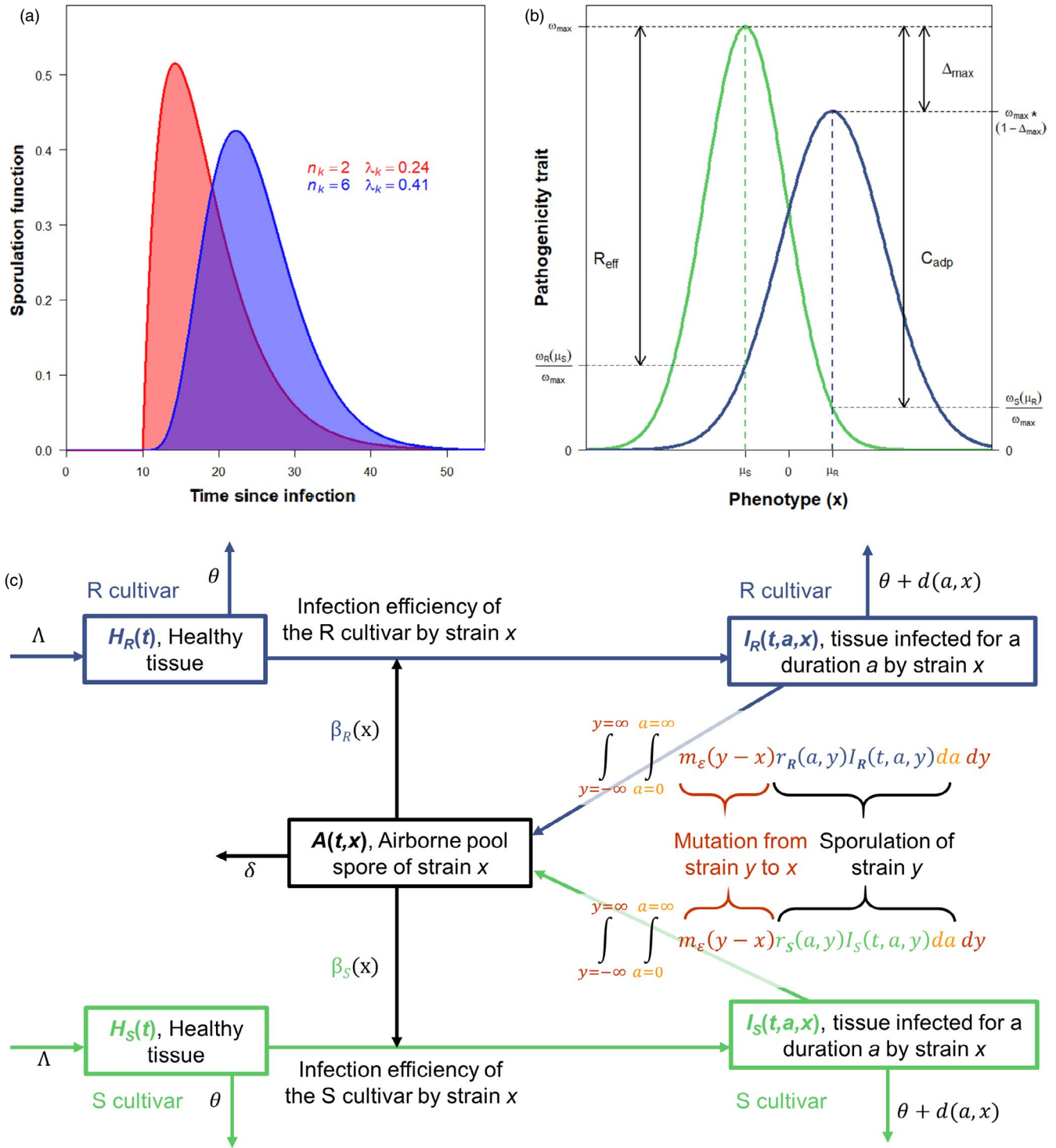
FIGURE 1 (a) Shapes of gamma sporulation function r_k(a, x) with latent period \tau_k = 10 and total spore production over the entire infectious period p_k = 5.94 as a function of n_k and \lambda_k . The infectious period is \cong 24 days for both functions. (b) Phenotypic landscapes of a pathogenicity trait \omega on a susceptible (S) and on a resistant (R) cultivar. Trait values are described by unnormalized Gaussian functions. The optimal parasite phenotypes \mu_S and \mu_R have maximum traits \omega_{max} and \omega_{max} (1 - \Delta_{max}) on the S and R cultivars, respectively. The relative effectiveness of resistance R_{eff} = (\omega_S(\mu_S) - \omega_R(\mu_S)) / \omega_{max} corresponds to the trait difference between the cultivars of phenotype \mu_S . The relative cost of adaptation C_{adp} = (\omega_S(\mu_S) - \omega_S(\mu_R)) / \omega_{max} corresponds to the trait difference between the phenotypes \mu_S and \mu_R on the S cultivar. Here, R_{eff} = 0.8 , C_{adp} = 0.9 , and \Delta_{max} = 0.2 . (c) Schematic representation of the model with 2 hosts (a susceptible (S) and a resistant (R) cultivar) and a one-dimensional mutation kernel (i.e., N_c = 2 and N = 1 ). All state variables and parameters are listed in Table 1
