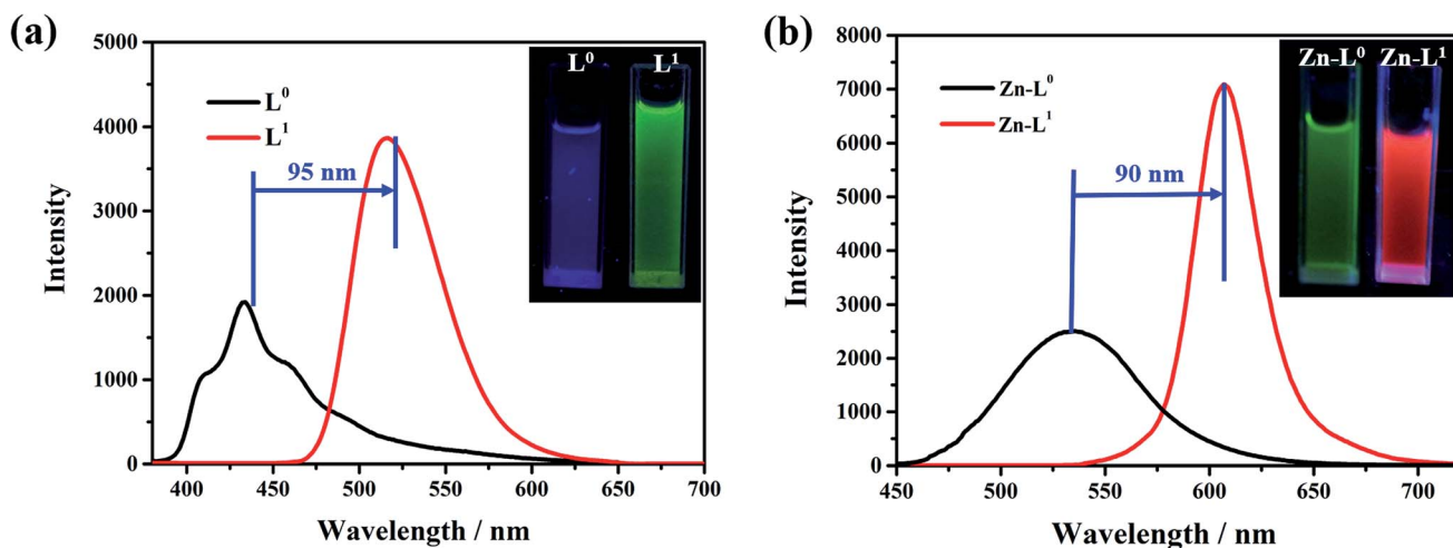
Fig. 3 PL spectra and photos of (a) L^0 and L^1 in THF with 5 \times 10^{-5} M ( L^0 : \lambda_{\text{ex}} = 420 nm; L^1 : \lambda_{\text{ex}} = 475 nm), (b) \text{Zn-L}^0 and \text{Zn-L}^1 in THF with 5 \times 10^{-5} M ( \text{Zn-L}^0 : \lambda_{\text{ex}} = 420 nm; \text{Zn-L}^1 : \lambda_{\text{ex}} = 475 nm). All photos were filmed at 365 nm in an ultraviolet light box.
