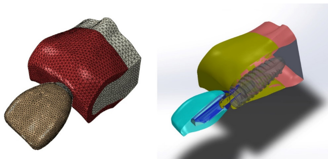
Figure 2. Implant model with the abutment, abutment screw, and crown in the anterior region of the maxilla.
