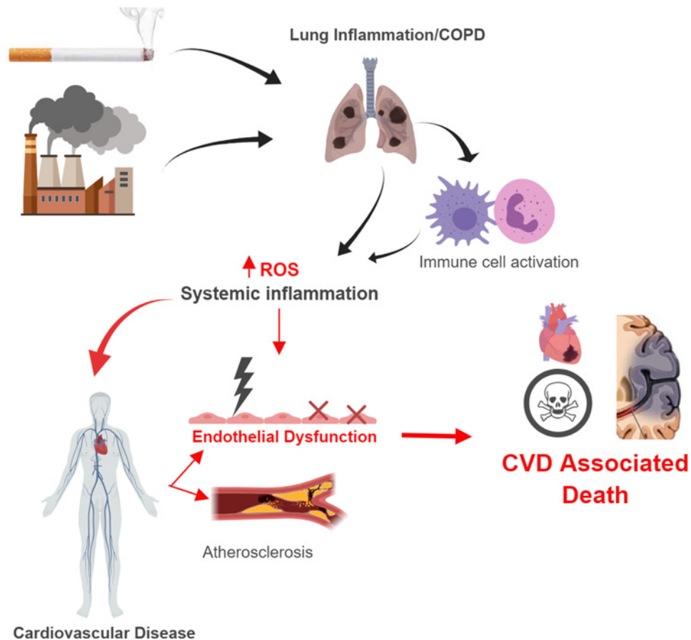
Figure 2. Schematic of lung inflammation and pathogenesis of COPD and comorbid CVD
