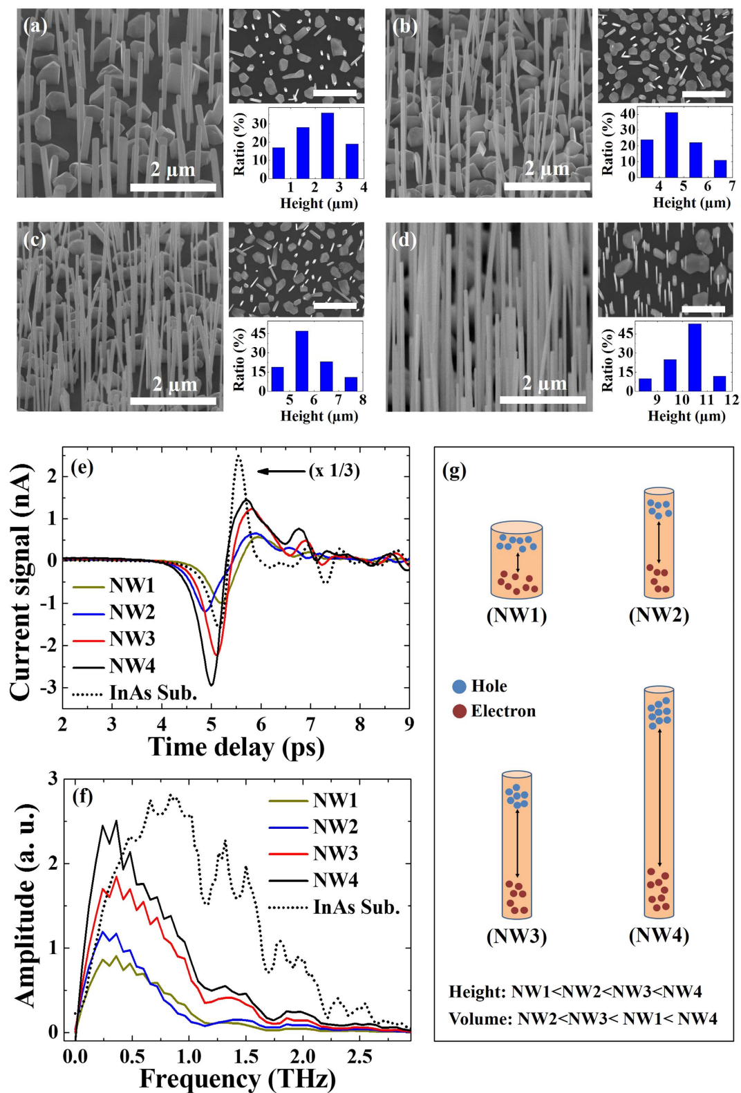
Figure 1. FE-SEM images of as-grown InAs NWs in the (a) NW1, (b) NW2, (c) NW3, and (d) NW4 samples, where each right-hand side shows a plan-view image (upper image, scale bar: 2 μm) and height distribution (bottom graph) of InAs NWs, (f) THz spectra obtained by applying FFT to the current signals of InAs NWs, and (g) schematic illustration of the carrier dynamics.
