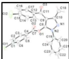
Fig. 1. The title molecule with the displacement ellipsoids shown at the 30% probability level.
