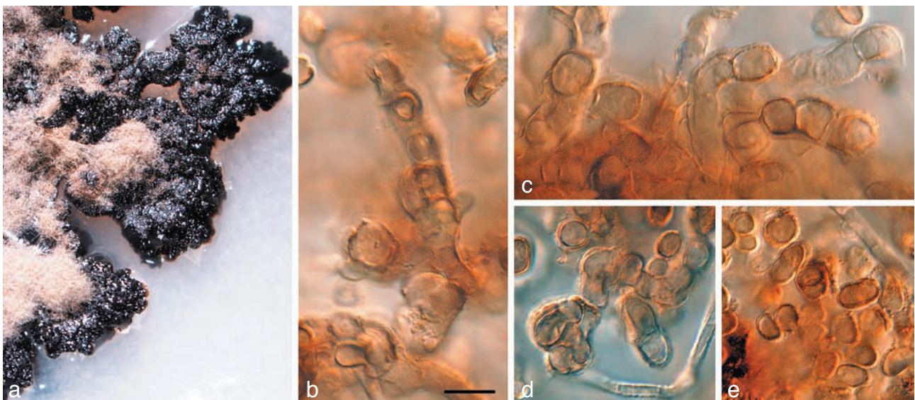
Fig. 6 Phaeothecoidea intermedia (CPC 13711). a. Colony on OA; b–d. hyphae giving rise to endoconidia; e. conidia. — Scale bar = 10 µm.
