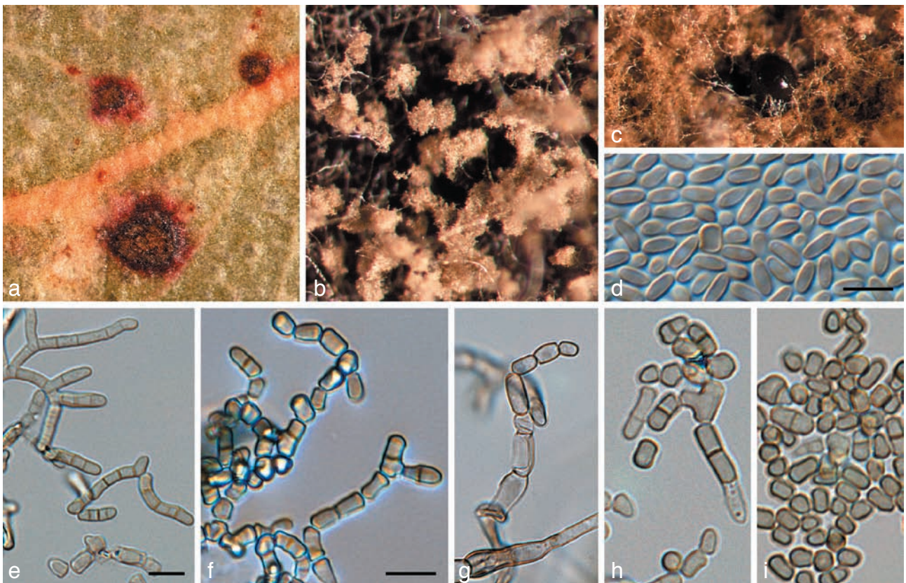
Fig. 9 Readeriella angustia (CPC 13608). a. Leaf spots; b. colony on PDA; c. Readeriella state among Cibissia conidiophores; d. Readeriella conidia; e–i. conidia of Cibissia state. — Scale bars = 10 \mu m.
