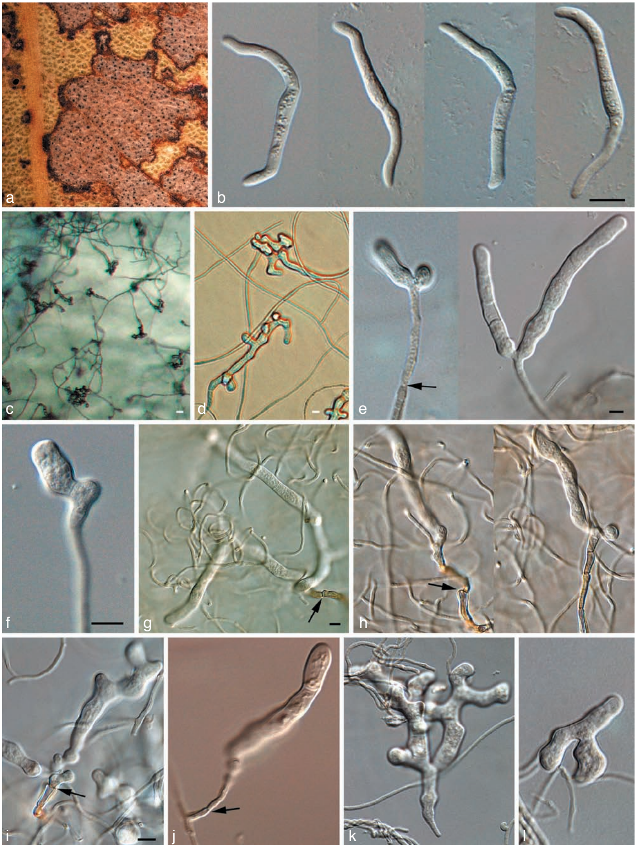
Fig. 21 Zasmidium aérohyalinosporum (CPC 14636). a. Leaf spot with black spermatogonia (small black dots); b. germinating ascospores on MEA; c–l. conidiogenous cells giving rise to conidia (arrow denotes point of attachment). — Scale bars = 10 µm.
