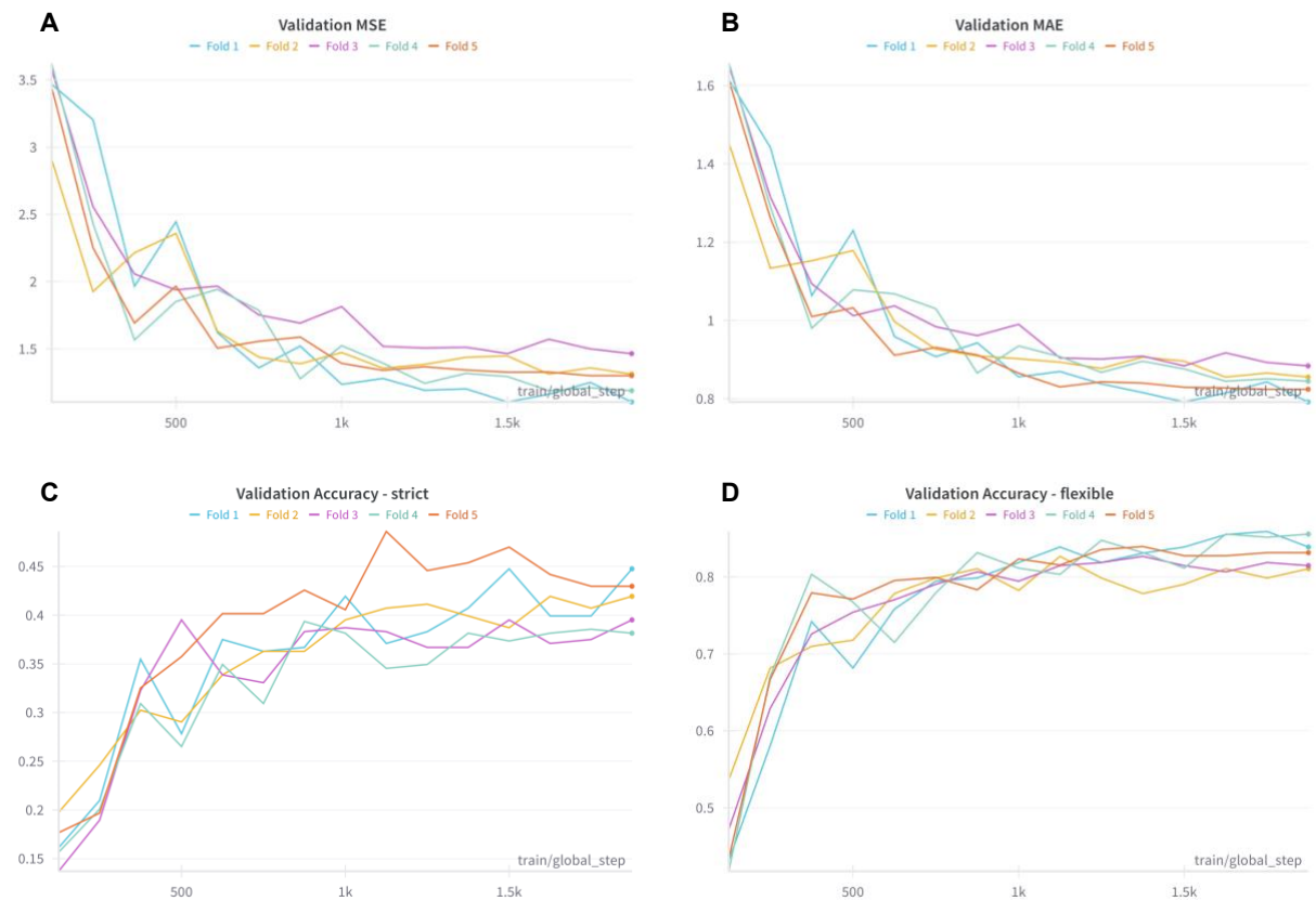
Supplementary Figure 2. (A) Validation Mean Squared Error (MSE), (B) Validation Mean Absolute Error (MAE), (C) Validation Accuracy strict, and (D) Validation Accuracy flexible
