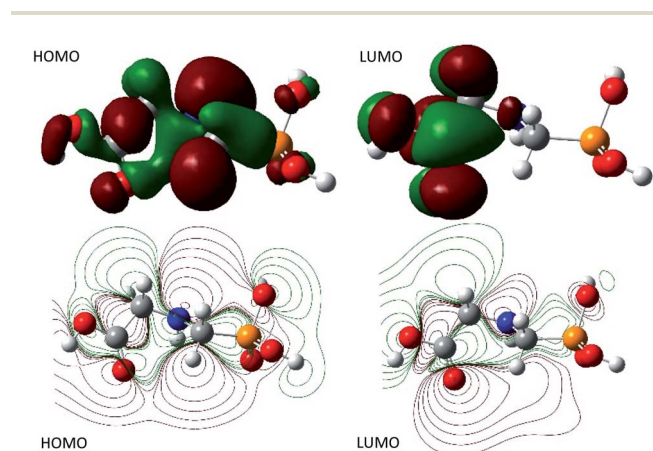
Fig. 4 HOMO and LUMO surfaces of gaseous GPS.
