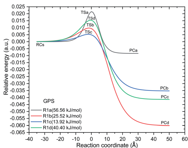
Fig. 7 Minimum energy potentials of the reaction of \cdot\text{OH} towards gas phase GPS. With the values of electronic energies at reaction complex (RC), transition state (TS), and product complex (PC), these potentials were interpolated by the Eckart unsymmetrical function. 30,31 The barrier height from the reaction complex of each reaction path are presented in parenthesis (at the bottom of well).
