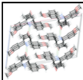
Fig. 2. Packing diagram showing the N-H...O hydrogen bonding (green dashed lines) parallel to the b-axis.
