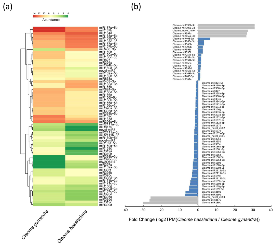
Figure 2. Expression patterns of miRNAs between Cleome gynandra and Cleome hassleriana . (a) Hierarchical cluster analysis of differentially expressed miRNAs between Cleome gynandra and Cleome hassleriana . The abundance used in the heatmap refers to the high (in red) and low (in green) expression levels of the miRNAs (TPM value of each miRNA). (b) Expression patterns of the differentially expressed miRNAs between Cleome gynandra and Cleome hassleriana . The color scales indicate the species-specific expressed miRNAs (grey bar) and non-species-specific expressed miRNAs (blue bar).
