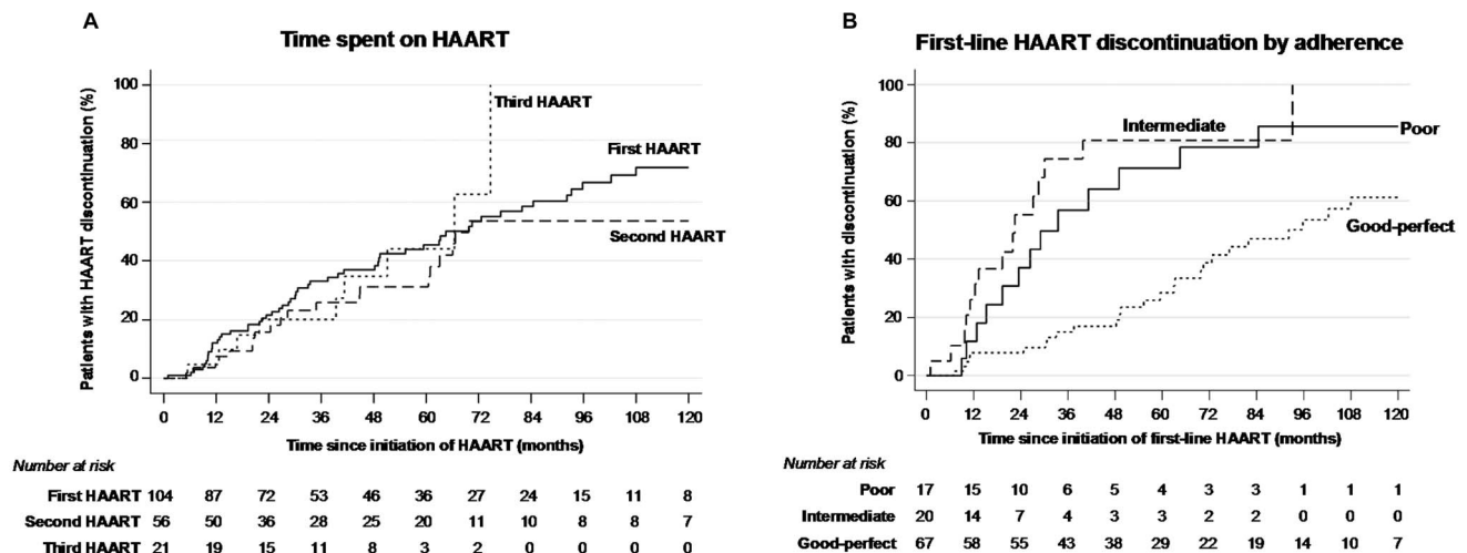
Figure 1. Kaplan–Meier survival curves for time spent on first vs. second vs. third HAART (A) and for time spent on first HAART by adherence to antiretrovirals (B). doi:10.1371/journal.pone.0096307.g001
