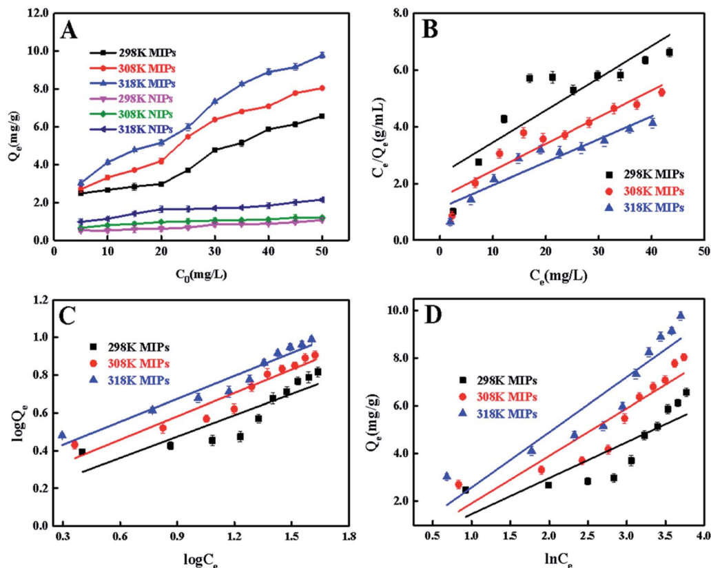
Fig. 5 (A) Static adsorption isotherms of 4-MDMC onto MIPs and NIPs at different temperatures; (B) Langmuir adsorption model, (C) Freundlich adsorption model, and (D) Temkin adsorption model of 4-MDMC onto MIPs at different temperatures.
