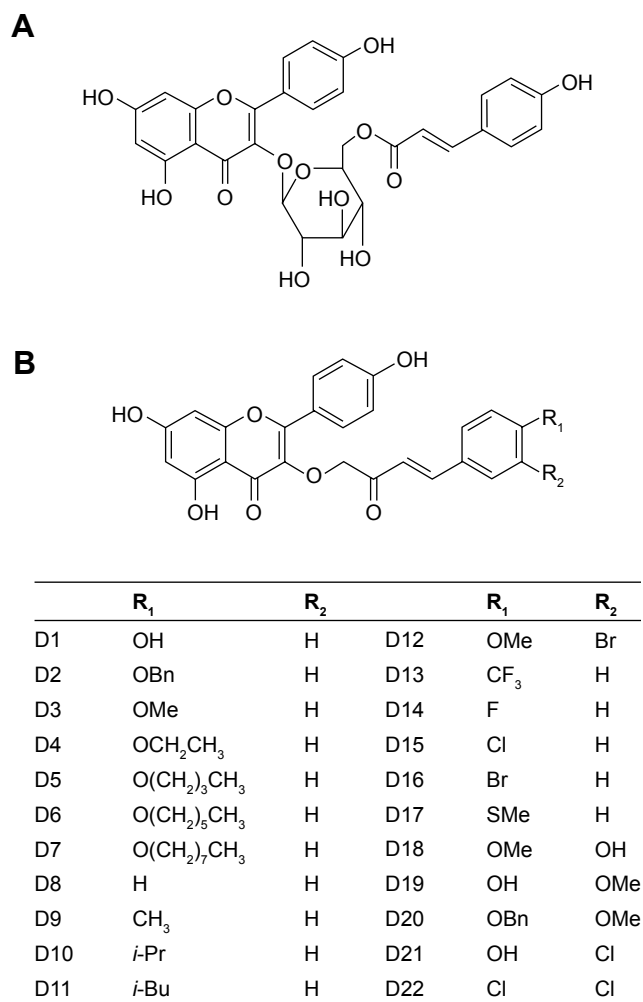
Figure 1 Chemical structures of tilioside (A) and 22 tilioside derivatives (B).
