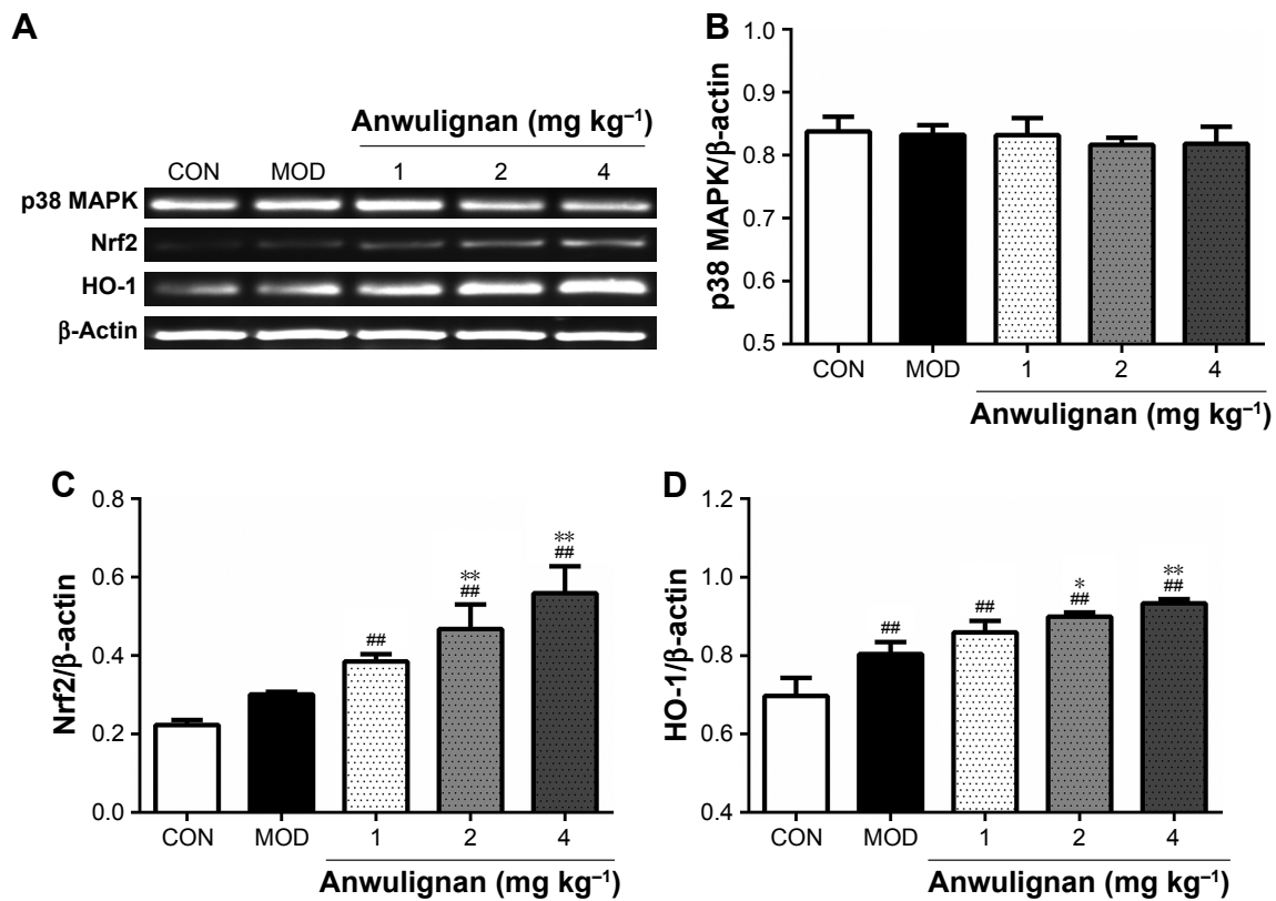
Figure 4 Effects of Anwulignan on the expressions of p38 MAPK, Nrf2, and HO-1 mRNA in the liver tissue of mice (mean \pm SD, n=3). Notes: (A) Agarose gel electrophoresis images of p38 MAPK, Nrf2, HO-1, and \beta -actin by RT-PCR. (B) Column charts of p38 MAPK/ \beta -actin by RT-PCR. (C) Column charts of Nrf2/ \beta -actin by RT-PCR. (D) Column charts of HO-1/ \beta -actin by RT-PCR. ### P <0.01, compared with the control group; * P <0.05, compared with the model group; ** P <0.01, compared with the model group. Abbreviations: MAPK, mitogen-activated protein kinase; CON, control; MOD, model; RT-PCR, reverse transcription-polymerase chain reaction.
