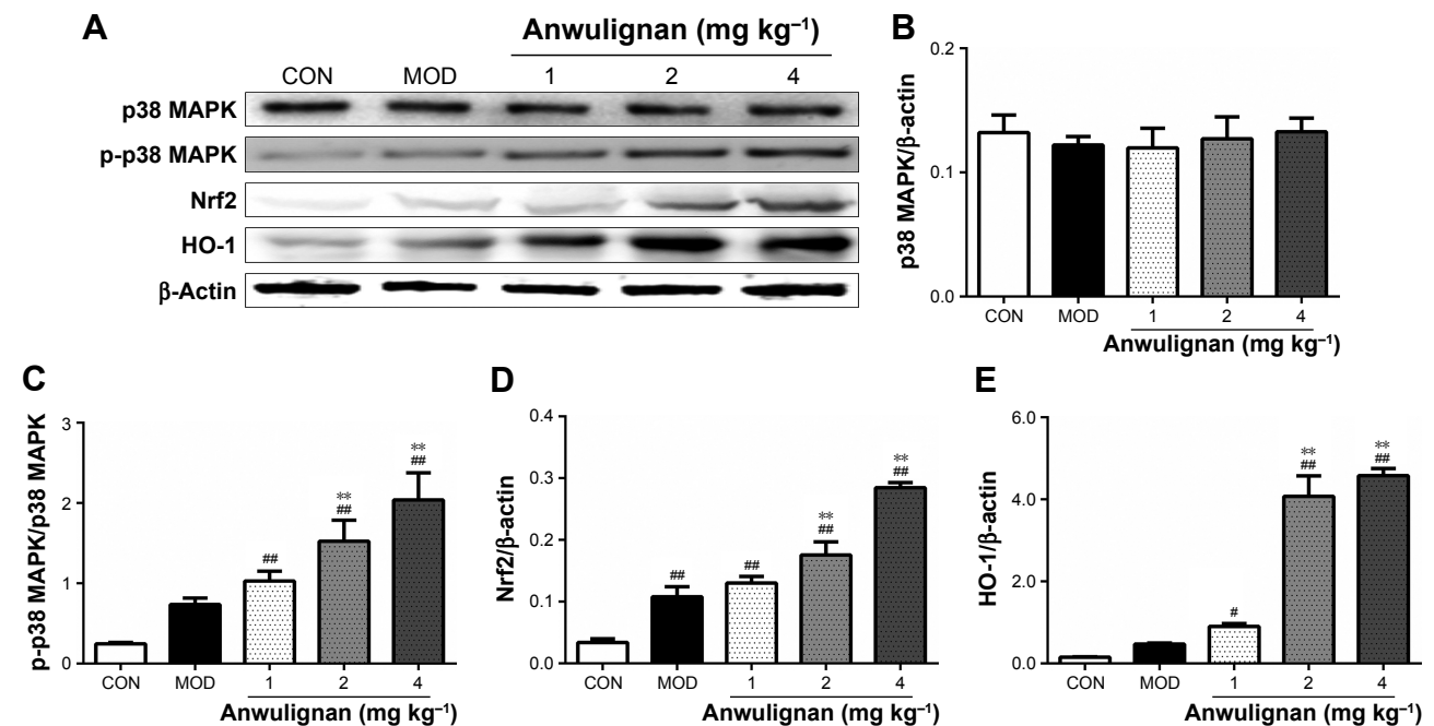
Figure 5 Effects of Anwulignan on the expressions of p38 MAPK, p-p38 MAPK, Nrf2, and HO-1 proteins in the liver tissue of mice (mean \pm SD, n=3). Notes: (A) p38 MAPK, p-p38 MAPK, Nrf2, HO-1, and \beta -actin protein electrophoresis images (Western blotting). (B) p38 MAPK/ \beta -actin column charts (Western blotting), (C) p-p38 MAPK/p38 MAPK column charts (Western blotting), (D) Nrf2/ \beta -actin column charts, and (E) HO-1/ \beta -actin column charts (Western blotting). * P <0.05, compared with the control group; ### P <0.01, compared with the control group; ** P <0.01, compared with the model group. Abbreviations: MAPK, mitogen-activated protein kinase; p-p38 MAPK, phosphorylation of p38 MAPK; CON, control; MOD, model.
