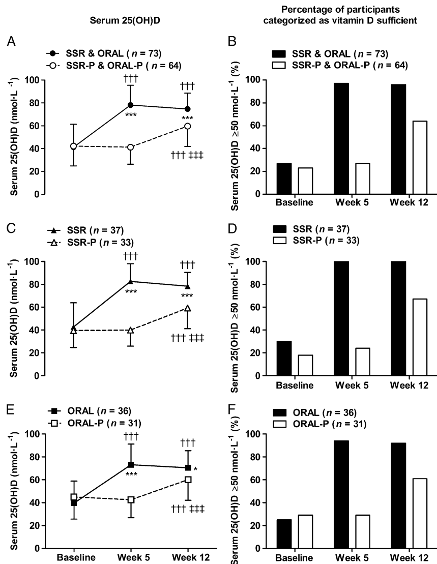
FIGURE 3 —Serum 25(OH)D and percentage of participants categorized as vitamin D sufficient (serum 25(OH)D \geq 50 nmol·L -1 ) in response to 12 wk of vitamin D supplementation by SSR and oral vitamin D 3 (ORAL). Panels A and B show combined active interventions (SSR and ORAL) vs combined placebo (SSR-P and ORAL-P), panels C and D show SSR vs SSR-P, and panels E & F show ORAL vs ORAL-P. ††† P < 0.001 , greater than baseline. †††† P < 0.001 , greater than week 5. * P < 0.05 and *** P < 0.001 , greater than placebo. Data in panels A, C, and E are mean \pm SD.
