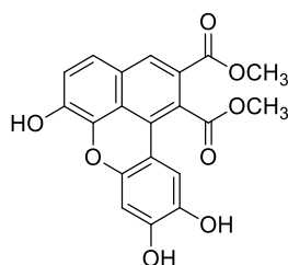
Figure 11. Dimethyl-6,9,10-trihydroxybenzol[k]xanthene-1,2-dicarboxylate 38.
