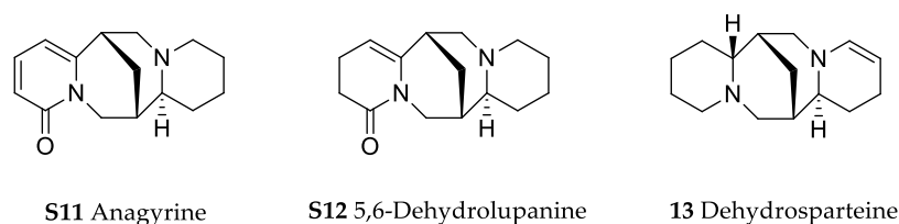
Figure 23. Quinolizidine alkaloids II, S11–S13.
