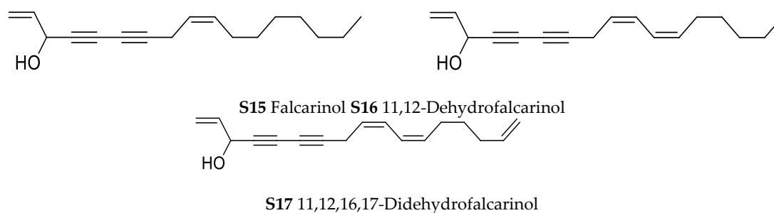
Figure 25. Polyacetylenes S15–S17.
