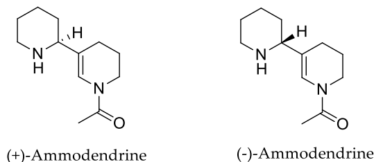
Figure 24. Piperidine alkaloid—Ammodendrine S14.
