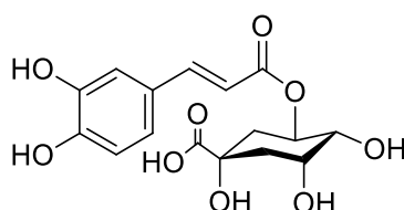
Figure 10. Chlorogenic acid (5-Caffeoyl quinic acid) 37.
