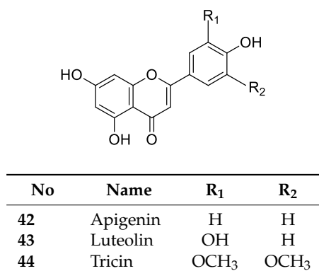
Figure 13. Flavones 42–44.
