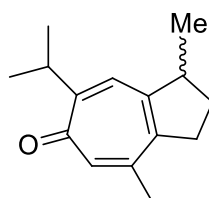
Figure 14. Tropone derivative—Orobanchone 45.
