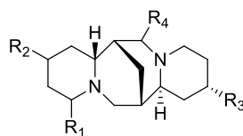
Figure 21. N-Methylangustifoline S1 .
