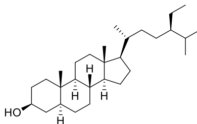
Figure 15. Sterols I: stigmastane derivative, stigmastanol 46.
