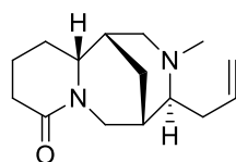
Figure 21. N-Methylangustifoline S1 .
