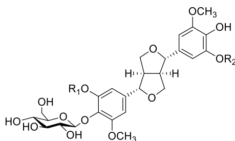
Figure 11. Dimethyl-6,9,10-trihydroxybenzol[k]xanthene-1,2-dicarboxylate 38.
