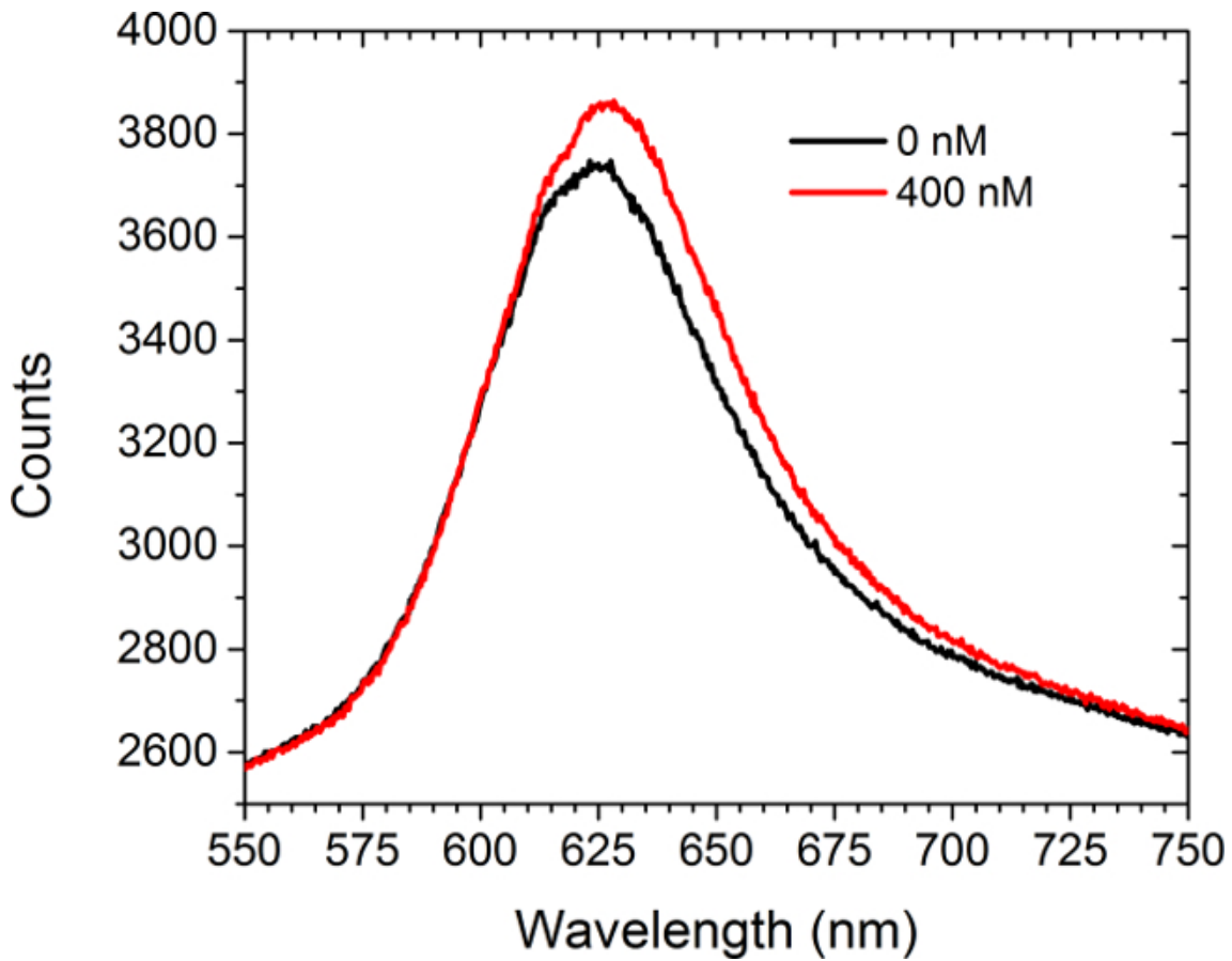
Figure 5. Spectral Modality. The spectra obtained from a c-myc functionalized array before and after the introduction of 400 nM solution of anti-c-myc antibodies. No cells were present in this study. Please click here to view a larger version of this figure.
