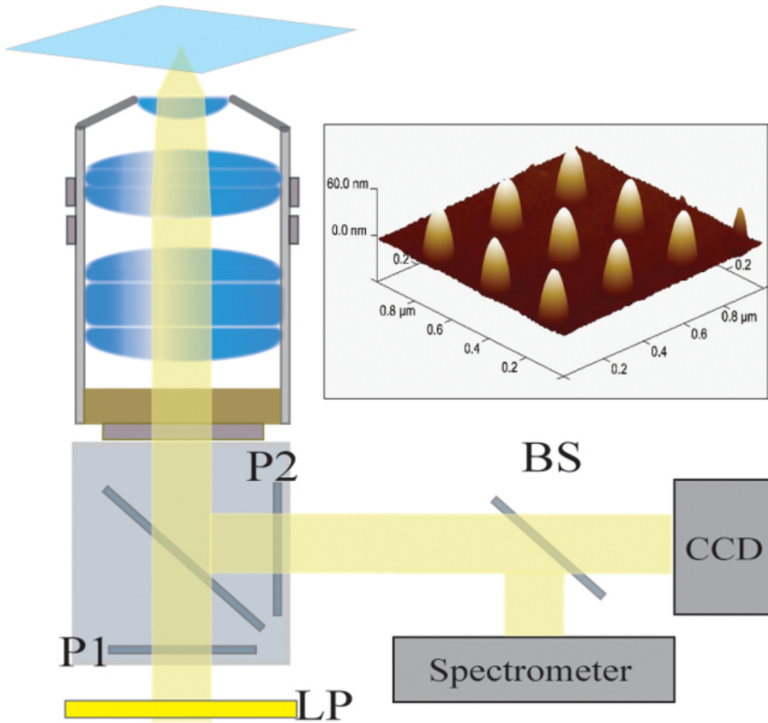
Figure 2. Optical Setup. The illuminated light from a halogen lamp is first filtered by a long pass filter (LP). The light is linearly polarized (P1) and illuminates the sample via a 40X/1.4 NA objective. The scattered light is collected by the objective and passed through a crossed polarizer (P2). A 50/50 beam splitter (BS) is inserted into the collected light path for simultaneous spectroscopic and imagery analysis. Top Right: An atomic force microscopy image of 9 individual nanostructures separated by a pitch of 300 nm. Please click here to view a larger version of this figure.
