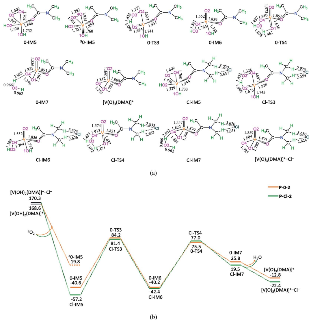
Fig. 3 The geometric structures (a) and the schematic energy diagrams (b) with the relative Gibbs free energy ( G_r , kJ mol -1 ) relative to the reactants for the oxidative dehydration of [V(OH) 2 (DMA)] + to [V(O) 3 (DMA)] + catalyzed by without/with Cl - in the DMA solution. For clarity, the hydrogen atoms on carbon are not shown. Bond lengths are reported in Å.
