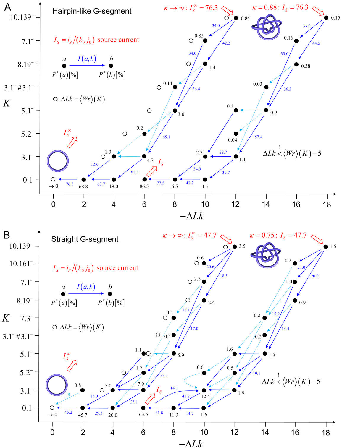
Figure 6. Comparison of NESS probabilities and probability currents generated by type-II topoisomerase activity with (A) hairpin and (B) straight G segment (74) in the state space spanned by knot type K and linking number \Delta Lk . In both cases, we imposed an external process that converts unknotted DNA with \Delta Lk = 0 to DNA forming a (source) knot K_S = 10.139^- with \Delta Lk_S = -12 in the limit of large source rate k_S (pathways shown on the left in (A) and (B)). Dominant probability currents with I_\infty(a, b)/I_S^\infty > 0.1 are shown as dark blue arrows and subdominant probability currents with 0.05 < I_\infty(a, b)/I_S^\infty < 0.1 are shown as light blue arrows. Steady-state probabilities P_\infty^*(K, \Delta Lk) , in percent, are shown next to each knot K . Open circles indicate positions of \Delta Lk = \langle Wr \rangle(K, \text{nicked}) , i.e., \Delta Lk_e = \Delta Lk - \langle Wr \rangle(K, \text{nicked}) = 0 (cf. white curve on the left in Figure 4). The pathways shown on the right in (A) and (B) show cases in which a supercoiled state is maintained by introducing the constraint \Delta Lk_e < -5 . In these cases, we assumed the presence of an external process that converts unknotted DNA with \Delta Lk = -6 to DNA forming a source knot K_S = 10.139^- with \Delta Lk_S = -18 , and the source rate k_S was adjusted to obtain the same source probability current I_S = 76.3 as for the pathway shown on the left to facilitate comparison.
