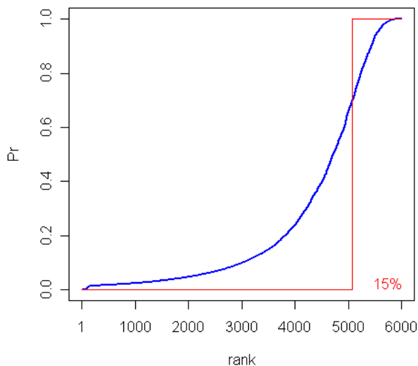
Figure 1 Probability of being periodic. The blue curve represents the probability of a gene being periodic ( Pr ) according to the model of [22]. The genes are sorted by probability values (rank) on the horizontal axis to facilitate the visualization. The red curve is the deterministic approximation using a 70% probability cutoff to consider a gene as periodic: \mathbb{P}(\text{gene}_i \text{ is periodic}) \geq 0.70 \Rightarrow \mathbb{P}(\text{gene}_i \text{ is periodic}) = 1 and \mathbb{P}(\text{gene}_i \text{ is periodic}) < 0.70 \Rightarrow \mathbb{P}(\text{gene}_i \text{ is periodic}) = 0 . This approximation labels 15% of the genes as periodic.
