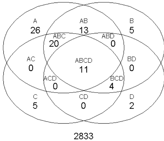
Figure 2 Venn diagram of over-represented terms. The Venn diagram shows the number of GO terms considered significantly over-represented ( p\text{-value} \leq 0.01 ) by the Fisher Exact Test using four different probability cutoffs \mathbb{P}(\text{gene}_i \text{ is periodic}) \geq A, B, C \text{ or } D \Rightarrow \text{periodic} : A = 0.70, B = 0.95, C = 0.99 and D = 0.9999 .
