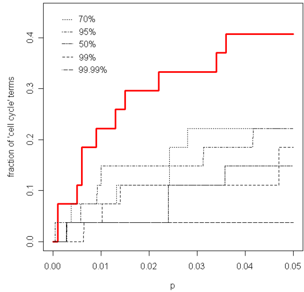
Figure 3 Fraction of "cell-cycle" GO terms selected as a function of the p-value. The curves show the fraction of GO terms containing the word "cell-cycle" in their definition that are considered significant as a function of the significance cutoff ( p ). The red curve is obtained with ProbCD and all others are obtained with one of the probability cutoffs: 50%, 70%, 95%, 99% or 99.99%.
